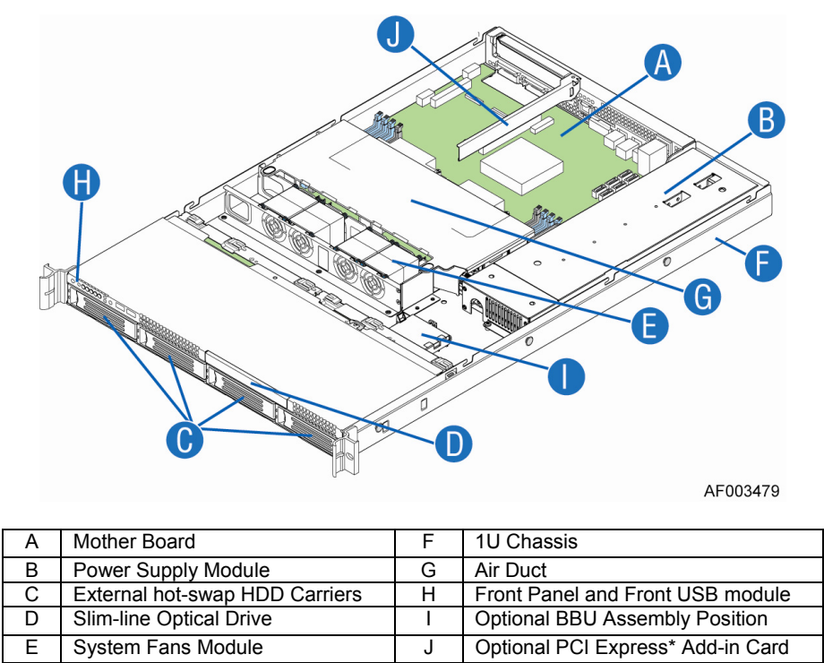
Figure 2. Major Chassis Components
