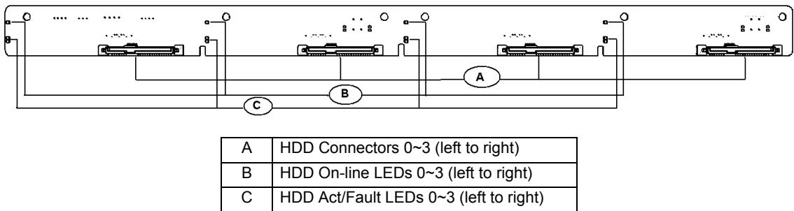
Figure 24. Backplane Component and Connectors (Front View)
