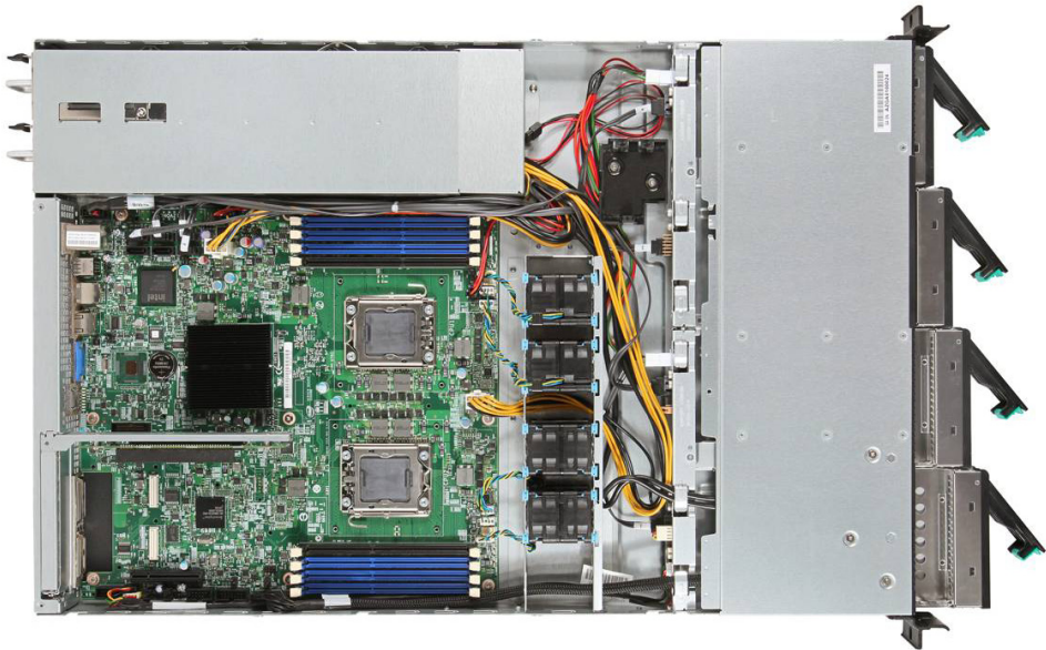
Figure 1. System Overview (HDD and Memory DIMMs are not included in package)
