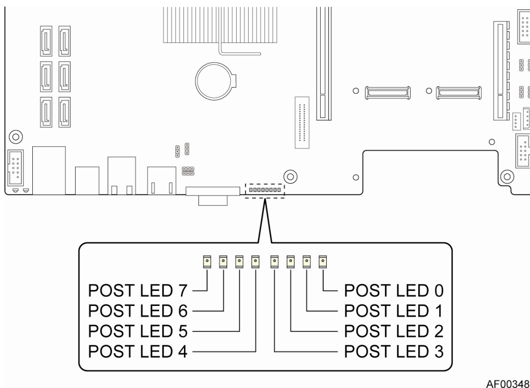
Figure 31. Diagnostic LED Placement Diagram
