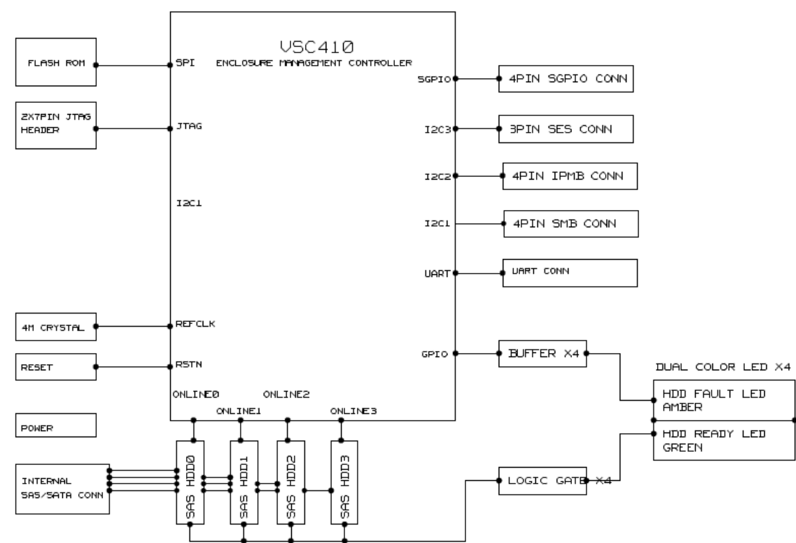
Figure 23. Passive Backplane Block Diagram
