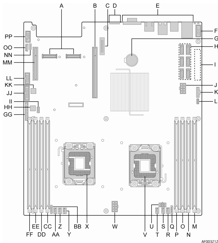
Figure 5. Intel® Server Board S5500WB 12V only Components
