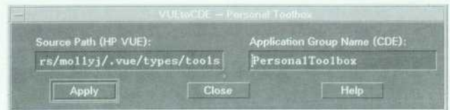
Fig. 9. Toolbox conversion.
