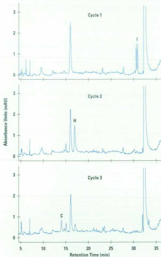
Fig. 11. High-sensitivity C-terminal sequencing of 50 picomoles of bovine beta-lactoglobulin A indicating approximately 50% recovery (24 picomoles) of cycle-1 isoleucine.
