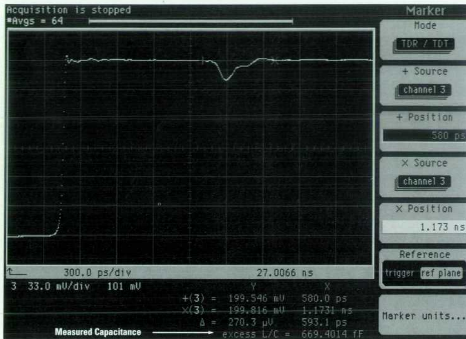
Fig. 15. Measuring the input capacitance of an HP 54701A active probe by placing cursors around the reflection caused by the probe.
