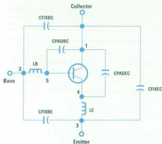
Fig. 12. Quarter device cell schematic of the SPICE file.
