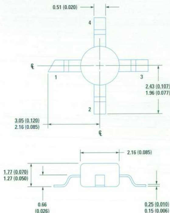
Fig. 7. Standard 86 package.
