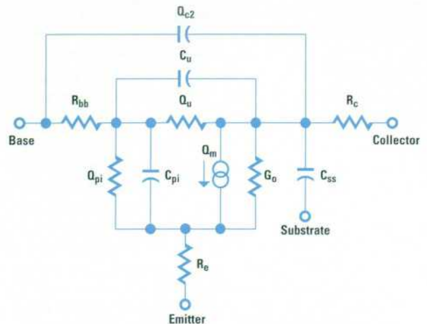
Fig. 9. Modified Gummel-Poon n-p-n ac model.
