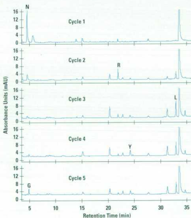
Fig. 8. Cycles 1 to 5 of C-terminal sequencing of 500 picomoles of recombinant beta-interferon applied to Zitex (230 picomoles of Asn recovered in cycle 1).
