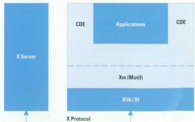
Fig. 1. CDE architecture.
