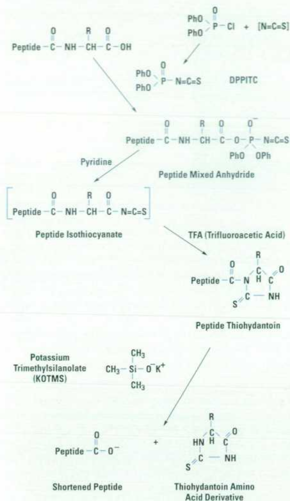
Fig. 3. Detailed reaction scheme of the HP thiohydantoin C-terminal sequencing chemistry. The chemical coupling reactions with diphenyl phosphorylisothiocyanate (DPPITC) generate a mixed anhydride followed by the extrusion of phosphate with ring formation to yield the peptide thiohydantoin. The subsequent chemical cleavage reaction with potassium trimethylsilanolate (KOTMS) releases the C-terminal amino acid thiohydantoin derivative (TH-aa) from the shortened peptide.
