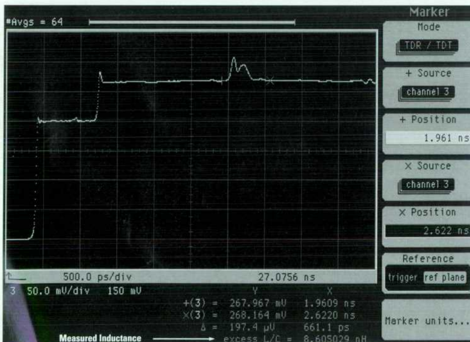
Fig. 16. Measuring the excess inductance of a connector in a 100-ohm system by placing cursors around the reflection caused by the inductance.
