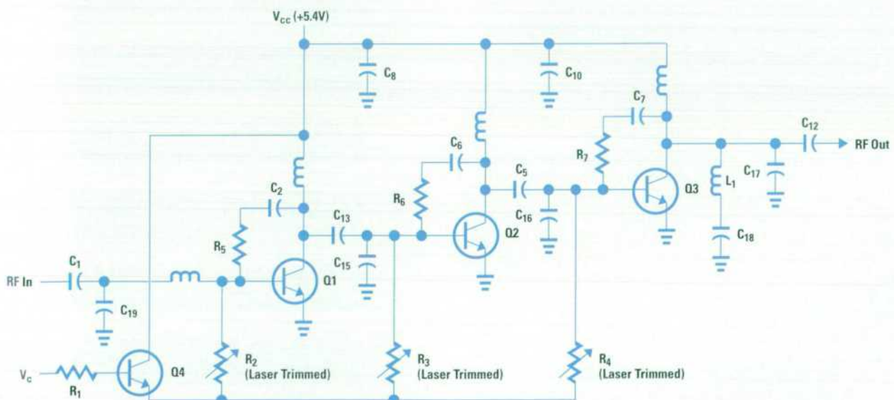
Fig. 3. Schematic diagram of the GSM power module.
