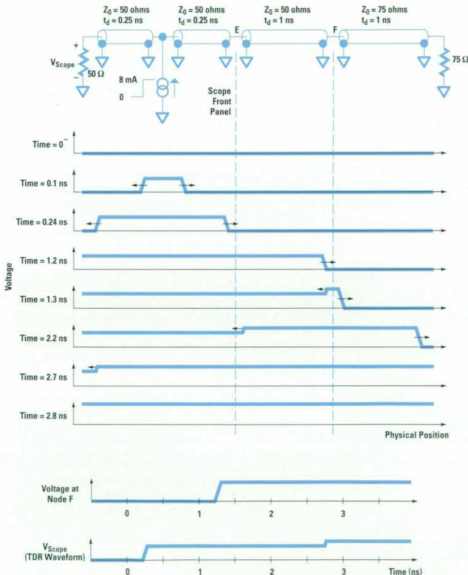
Fig. 4. Typical measurement setup and waveforms for an oscilloscope with an internal time-domain reflectometer (TDR).
