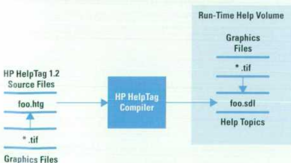
Fig. 9. The HelpTag compilation process.
