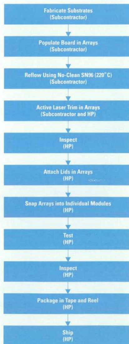
Fig. 5. Volume assembly process flow.
