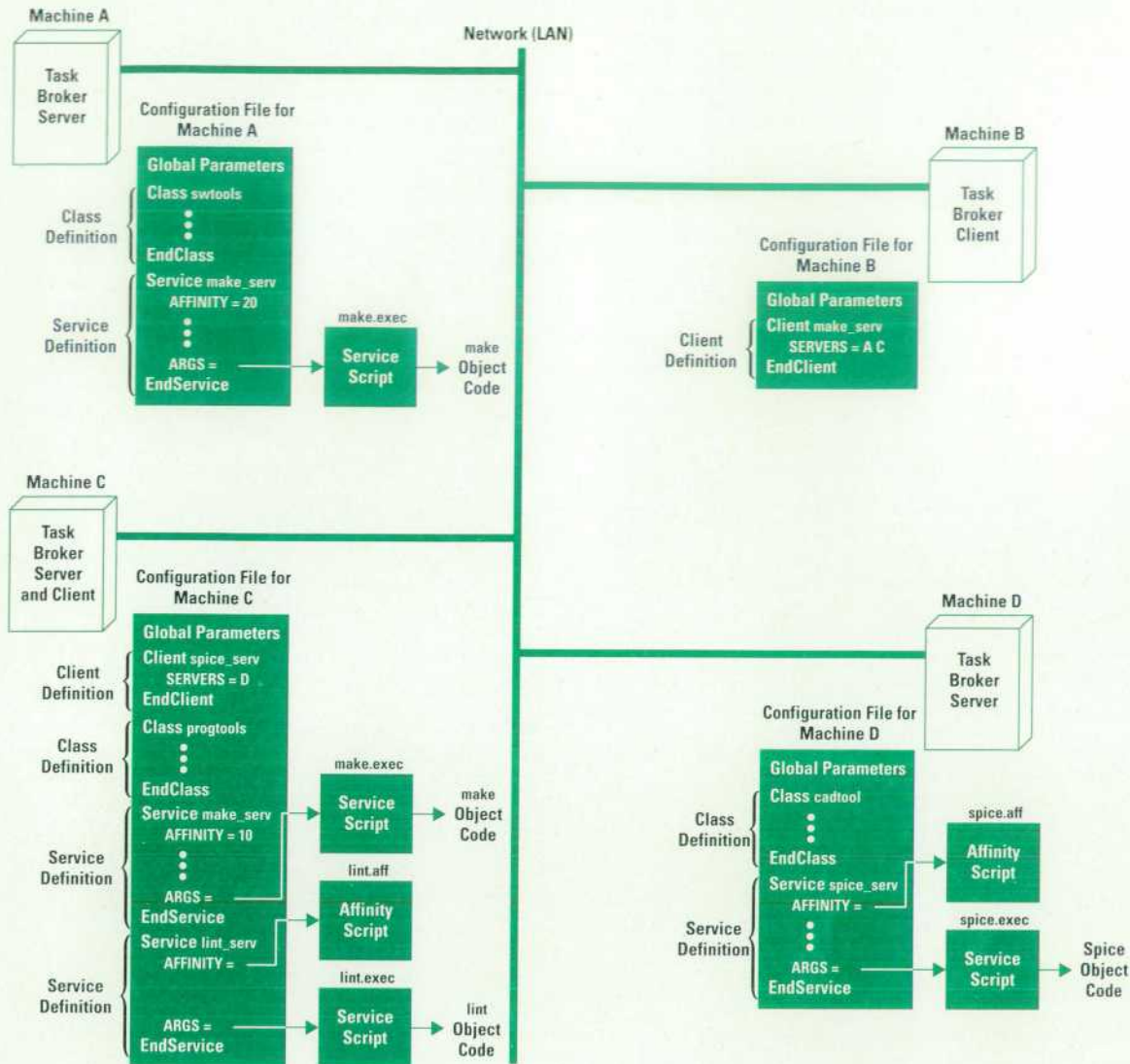
Fig. 1. An overview of Task Broker configuration files.
