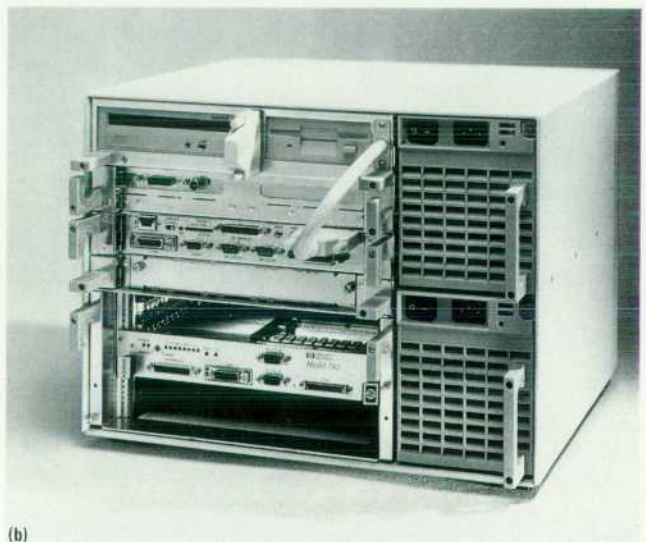
Fig. 1. (a) The HP 9000 Model 742rt board-level computer. (b) An HP 9000 Model 747i industrial workstation with a Model 742rt loaded in.
