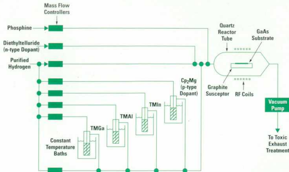
Fig. 3. Simplified schematic diagram of an organometallic vapor phase epitaxy (OMVPE) reactor.
