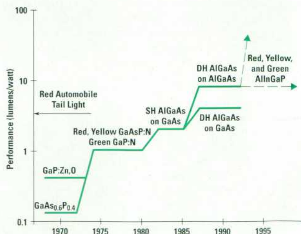
Fig. 1. Time evolution of light-emitting diode technology.
