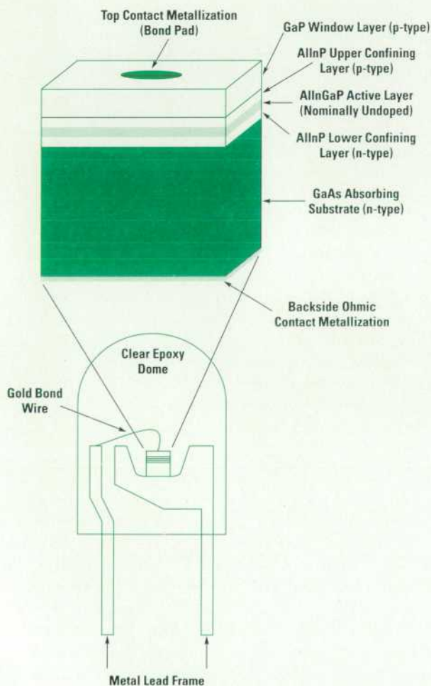
Fig. 4. AlInGaP LED structure.
