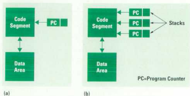
Fig. 4. Thread configurations. (a) A typical single-thread process. (b) A multiple-thread process.
