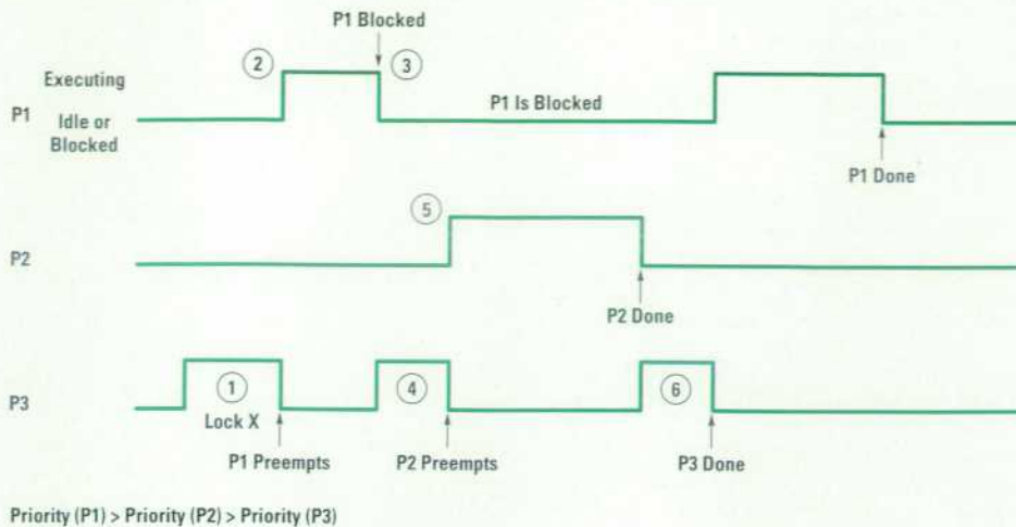
Fig. 7. A time line illustrating priority inversion.
