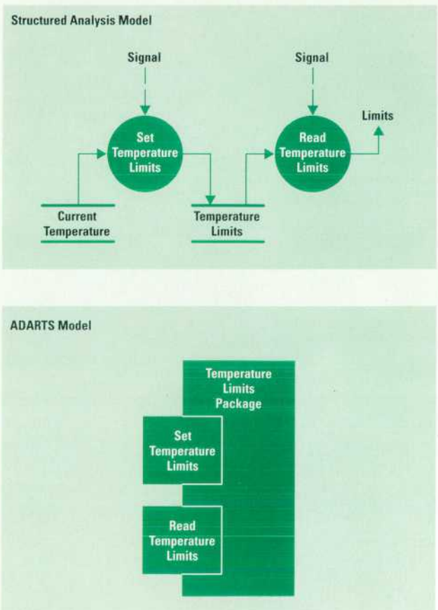
Fig. 8. A model of a data abstraction package.
