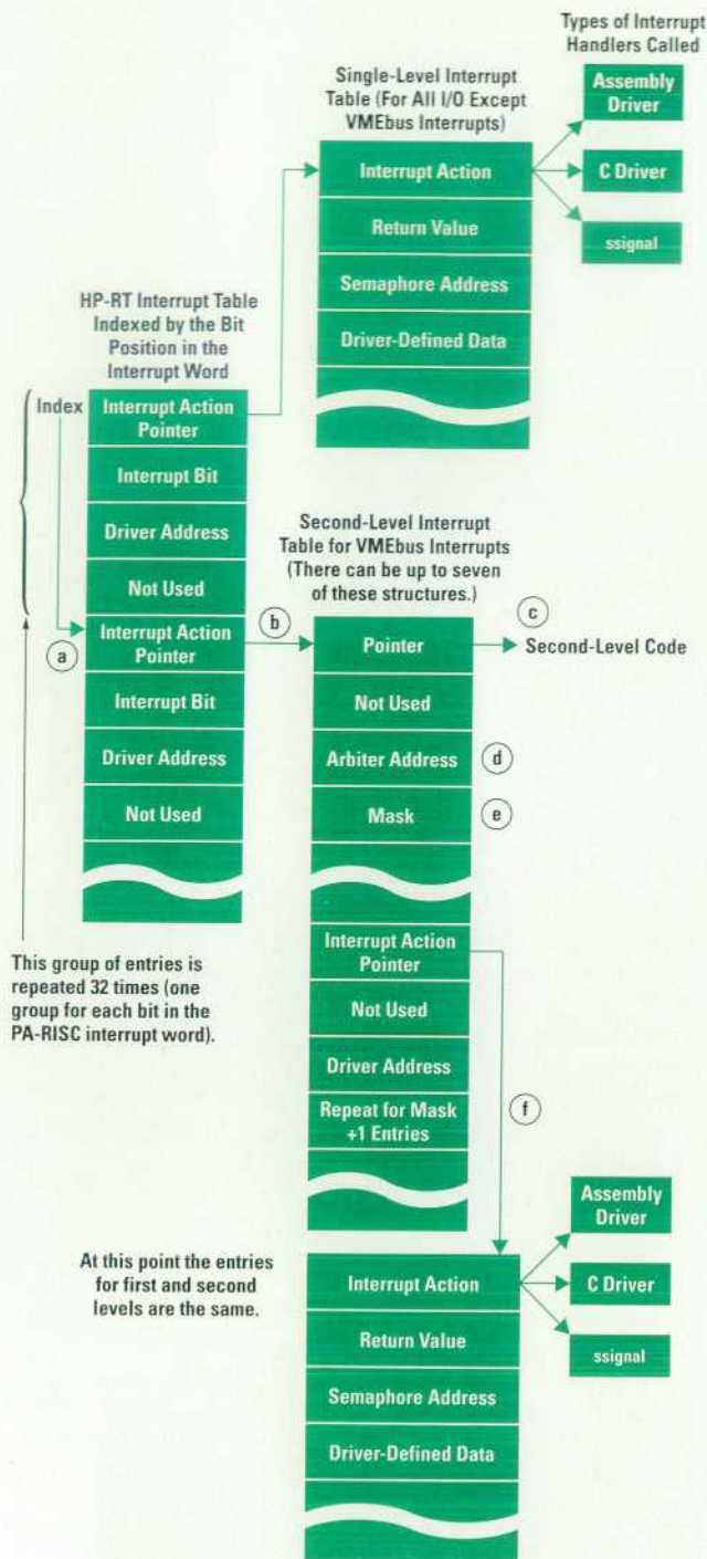
Fig. 3. The HP-RT interrupt table structure.
