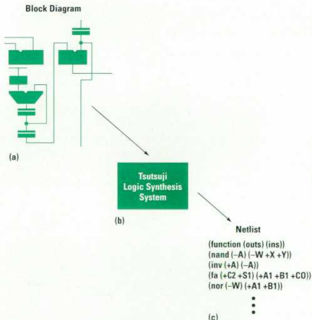
Fig. 1. Tsutsuji is a high-performance logic synthesis system. Designs are expressed as block diagrams, which are transformed by Tsutsuji into a netlist file that can be used by gate array manufacturers to produce an application-specific integrated circuit (ASIC).
