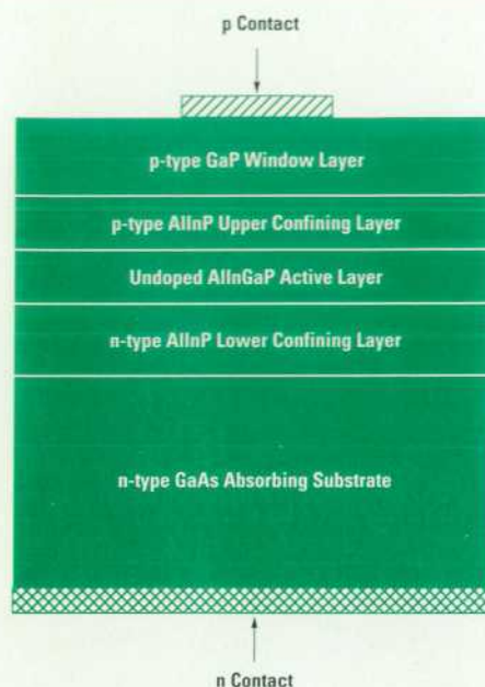
Fig. 5. AlInGaP double-heterostructure LED on an absorbing substrate.
