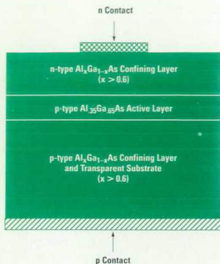
Fig. 4. AlGaAs double-heterostructure LED on a transparent substrate.
