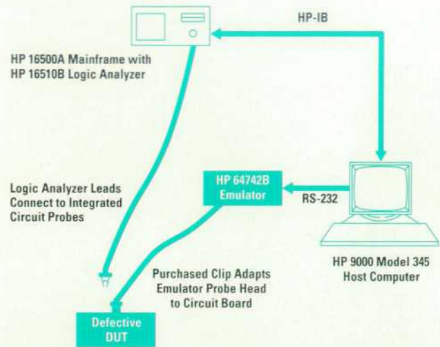
Fig. 1. System used in HP 54600 Series oscilloscope production to troubleshoot defective digital boards.
