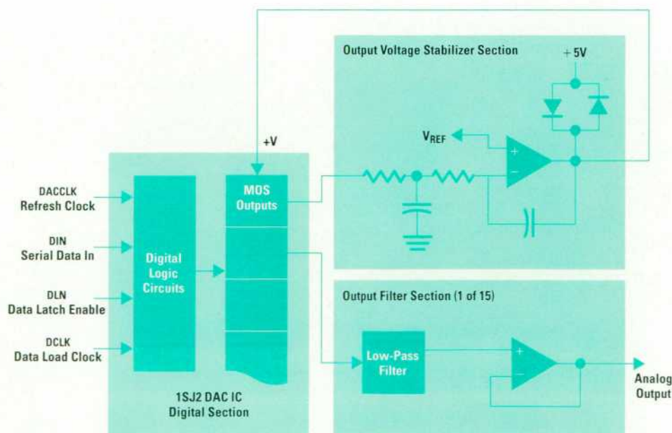
Fig. 1. Block diagram of the high-resolution, multichannel, indirect type digital-to-analog converter.
