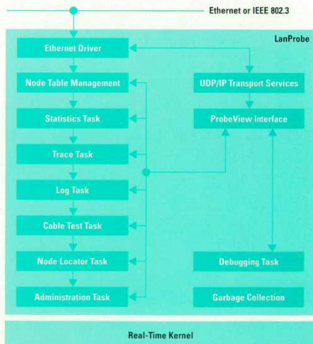
Fig. 8. HP LanProbe internals and tasks.
