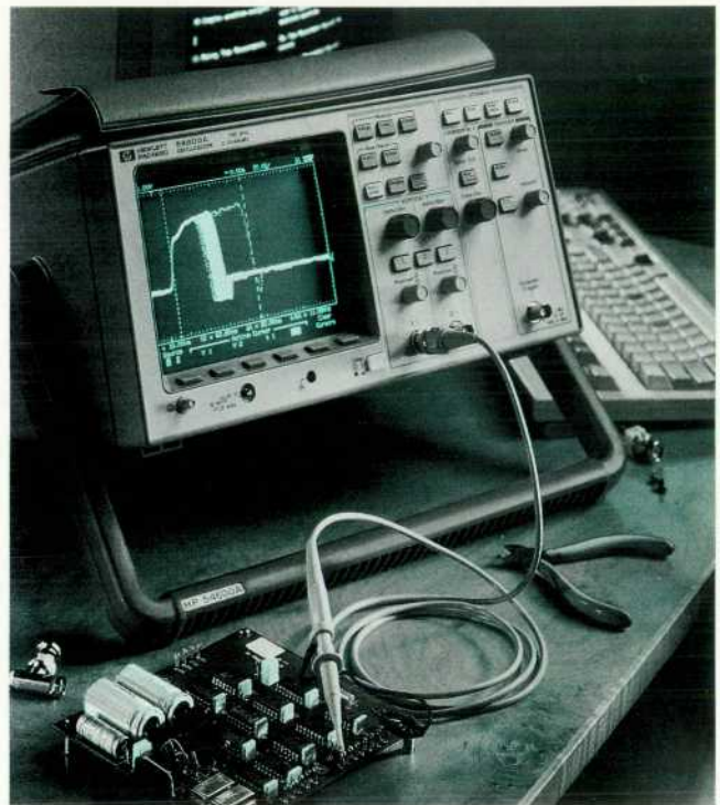
Fig. 1. The HP 54600A is a two-channel 100-MHz general-purpose digitizing oscilloscope.
