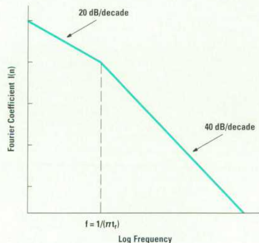
Fig. 6. The envelope of the Fourier series of a trapezoidal waveform has a breakpoint that depends purely upon the rise time ( t_r ). Slowing down the rise time shifts this breakpoint down in frequency and reduces the amplitude of the high-frequency harmonics.
