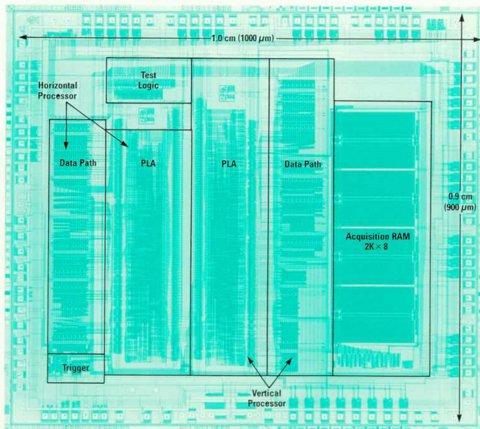
Fig. 6. Acquisition processor chip layout.
