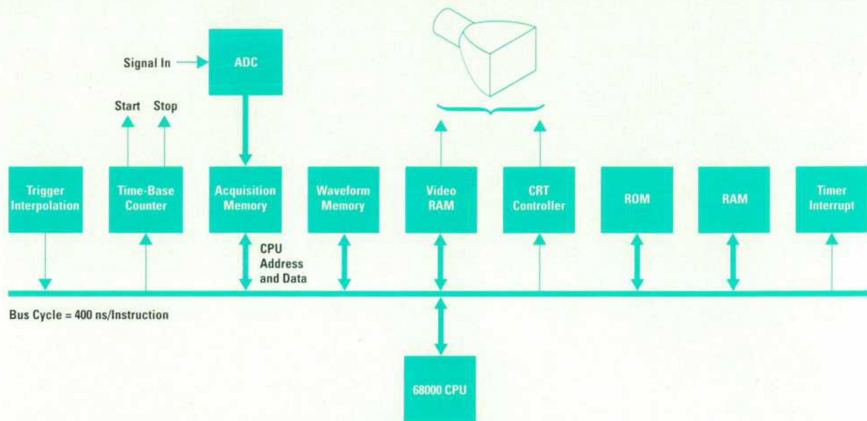
Fig. 1. Previous raster digital oscilloscope architecture, simplified.
