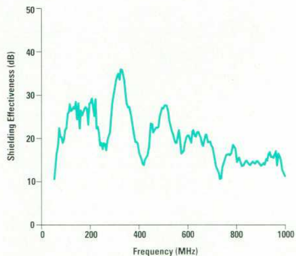
Fig. 3. Measured shielding effectiveness of the HP 54600 oscilloscope enclosure including seams and apertures. The harmonic comb generator was used to obtain the plot.
