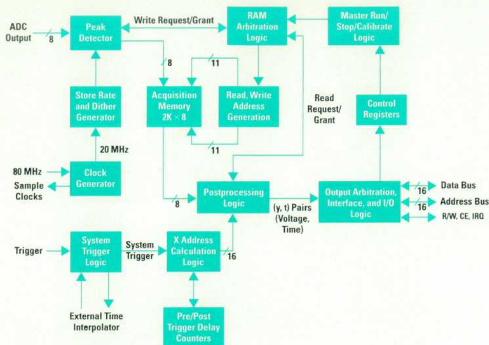
Fig. 5. Logical block diagram of the acquisition processor.
