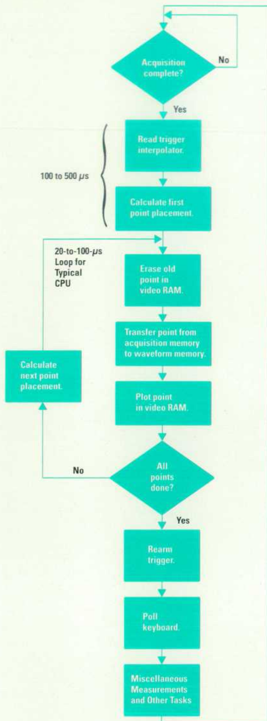
Fig. 2. Simplified task flows in the previous raster digital oscilloscope architecture.
