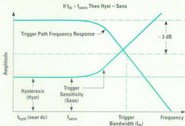
Fig. 5. Frequency response curve showing the area where hysteresis can be used as a measure of trigger sensitivity.
