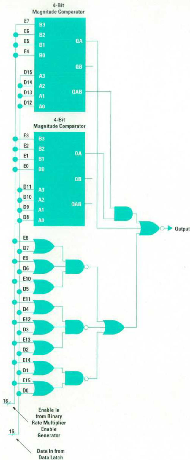
Fig. 7. Modified binary rate multiplier.
