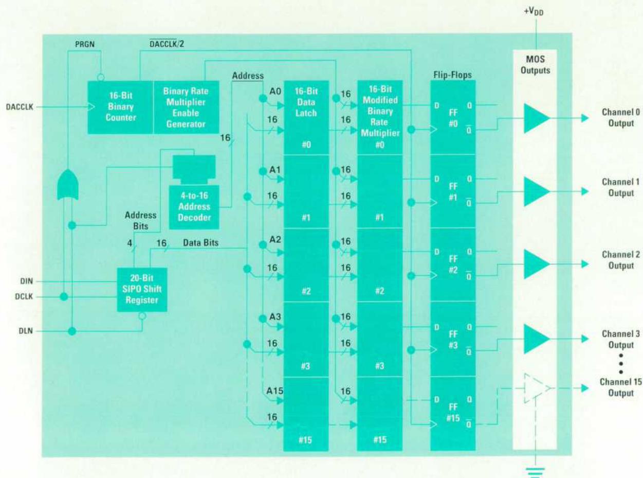
Fig. 4. Block diagram of the 1SJ2 integrated circuit, which is the digital section of the multichannel DAC.
