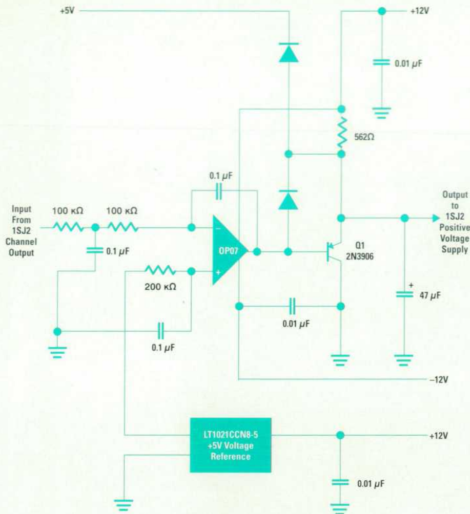
Fig. 8. DAC output voltage stabilizer.
