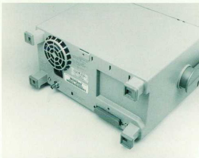
Fig. 3. Two screws allow removal of the chassis assembly from the cabinet. For ruggedness, the rear feet are integrated into the cabinet and have four load-bearing walls.
