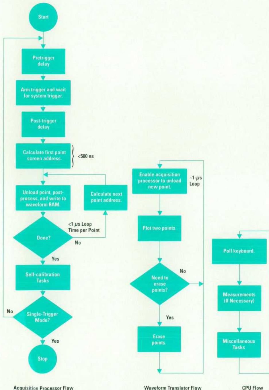
Fig. 4. Simplified task flows in the new raster digital oscilloscope architecture.
