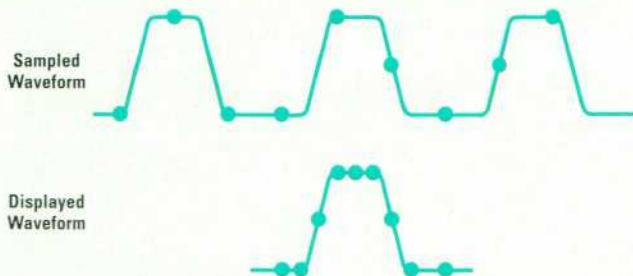
Fig. 1. Random repetitive sampling.
