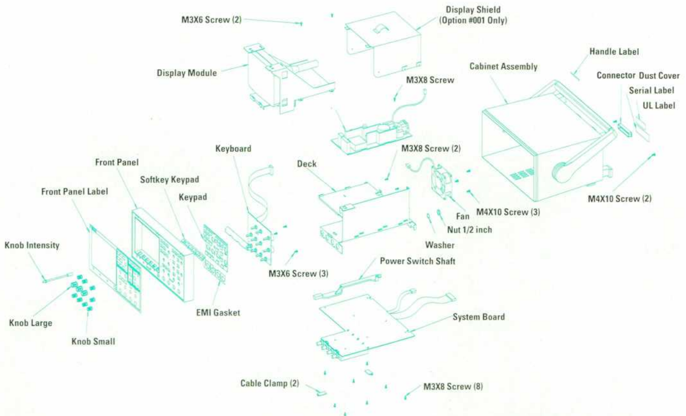
Fig. 1. The components of the final assembly process of the HP 54600 Series oscilloscopes. Only 22 threaded fasteners are used.
