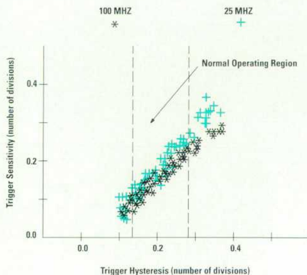
Fig. 6. Plot showing the linear relationship between hysteresis and trigger sensitivity.
