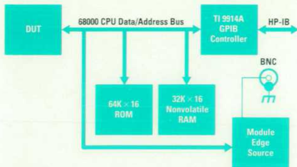
Fig. 2. Block diagram of the production calibration module.
