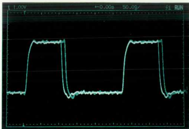
Fig. 1. Comparison of an autostored good unit signal at half intensity with a bad unit signal at full intensity.
