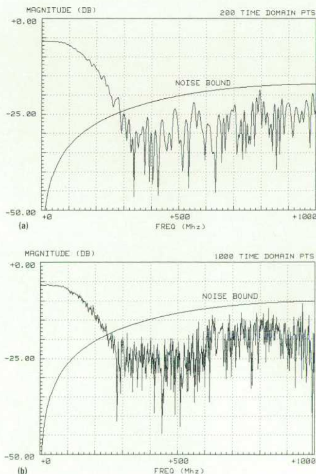
Fig. 3. Noise in the frequency response of an HP 54600A. (a) 200 points. (b) 1000 points.
