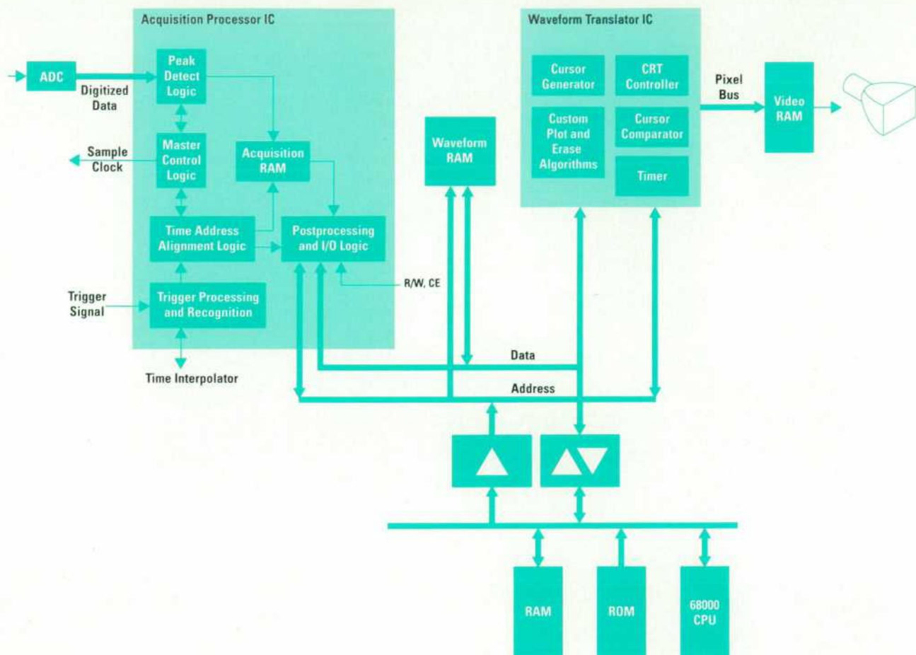
Fig. 3. New raster digital oscilloscope architecture.
