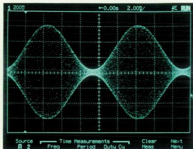
Fig. 2. The waveform processing technology used in the HP 54600 family of oscilloscopes accurately displays complex waveforms such as amplitude modulated signals.
