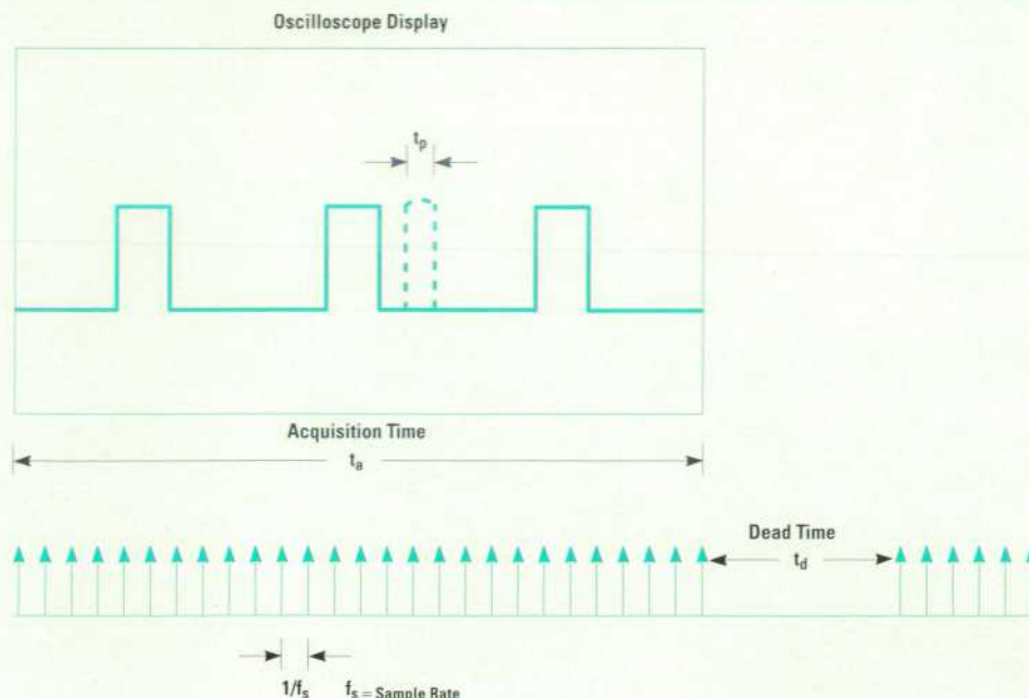
Fig. 3. Acquisition time, sample rate, and dead time.
