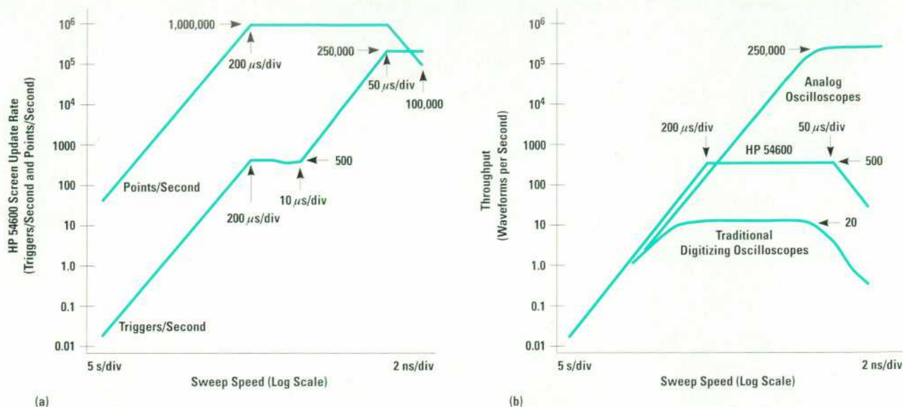
Fig. 8. (a) HP 54600 screen update rate. (b) HP 54600 throughput compared to analog oscilloscopes and traditional digitizing oscilloscopes.
