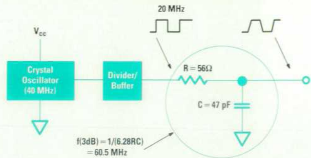
Fig. 5. An RC filter is installed following the microprocessor divider/buffer circuit. The filter slows down the rise time of the clock signal and greatly reduces the clock harmonics.
