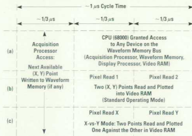
Fig. 7. Waveform memory bus arbitration.
