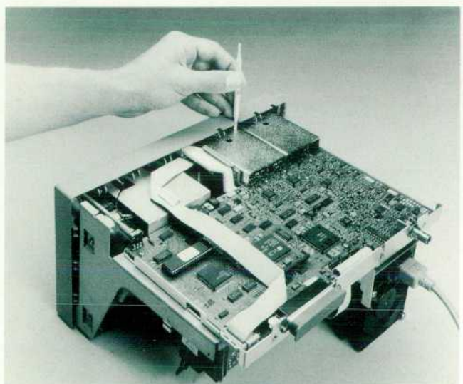
Fig. 4. With the cabinet removed, four holes in the front panel allow calibration for flatness and overshoot.
