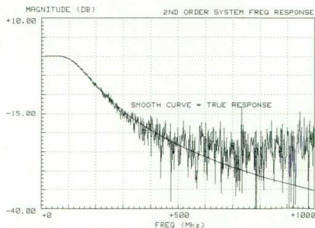
Fig. 5. True frequency response of a second-order system compared with the estimated response.
