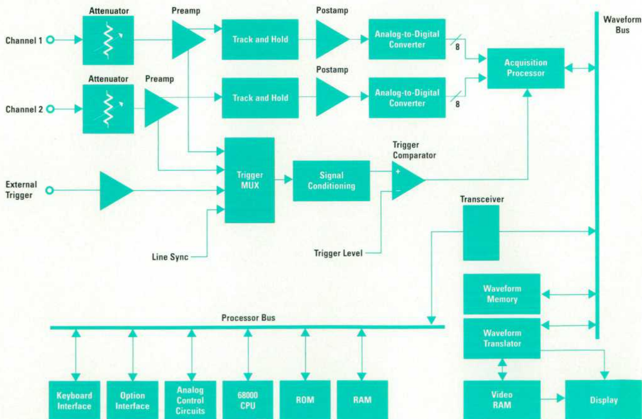
Fig. 5. Simplified block diagram of the HP 54600A two-channel oscilloscope.
