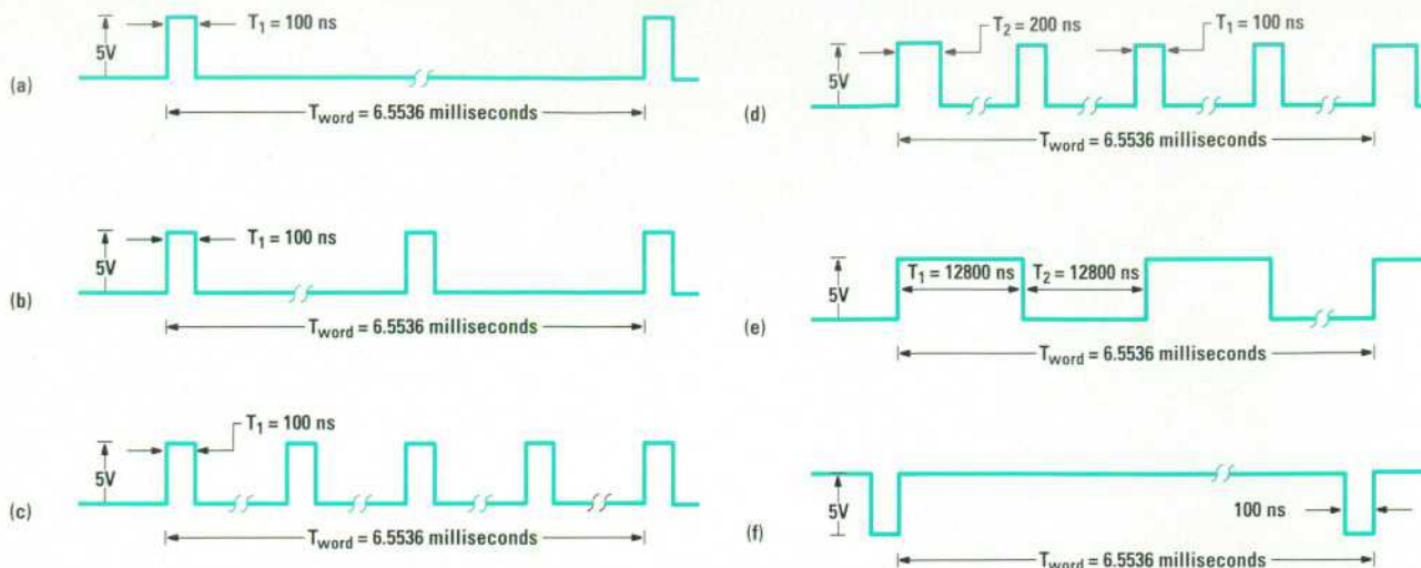
Fig. 5. 1SJ2 DAC IC output for 16-bit data and a 20-MHz DACCLK frequency. (a) D0 only high gives one 5V, 100-ns pulse per T_{\text{word}} period. (b) D1 only high gives two 5V, 100-ns pulses per T_{\text{word}} period. (c) D8 only high gives 256 5V, 100-ns pulses per T_{\text{word}} period. (d) D8 and D0 only high gives 255 5V, 100-ns pulses and one 5V, 200-ns pulse per T_{\text{word}} period. (e) D15 only high gives 256 5V, 12800-ns pulses per T_{\text{word}} period (50% duty cycle). (f) D0 through D15 all high gives one 5V, 6.5535-ms pulse per T_{\text{word}} period.
