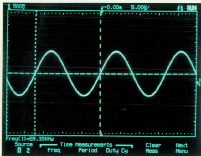
Fig. 4. The oscilloscope automatically measures the frequency of a sine wave and places the cursors automatically to show the measurement location on the waveform.
