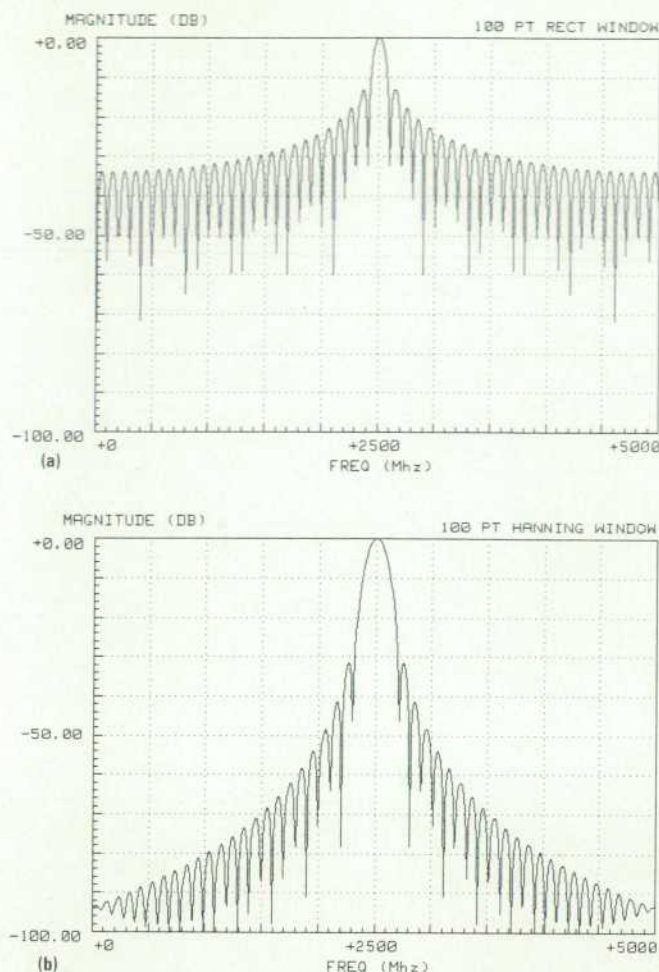
Fig. 7. Frequency spectrum for (a) a 100-point rectangular window and (b) a 100-point Hanning window.
