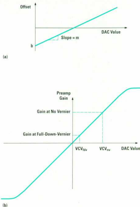
Fig. 2. (a) Offset voltages are generated by the DAC from an equation of the form y = mx + b . (b) Preamp gain as a function of DAC value.
