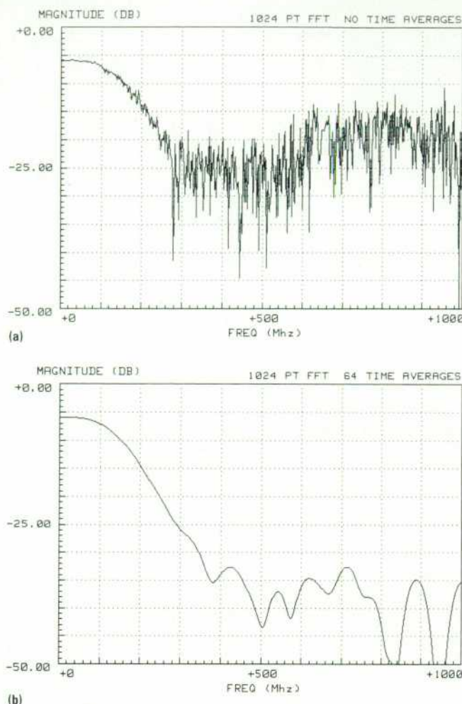
Fig. 4. Noise in the frequency response of an HP 54600A. (a) No averages. (b) 64 averages.
