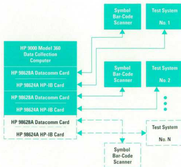
Fig. 8. Data collection scheme for the HP 54600 production test system.
