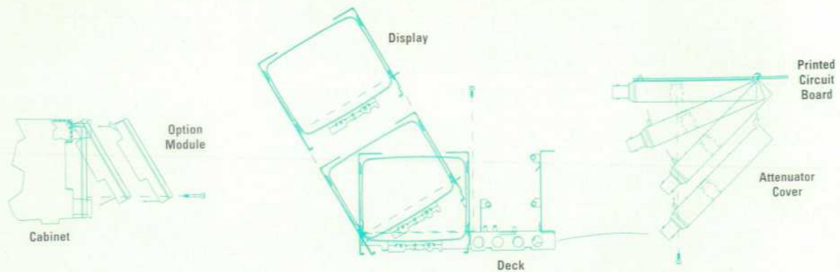
Fig. 2. Examples of HP 54600 assembly techniques.
