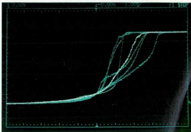
Fig. 3. Power-up characteristics of a power supply over the specified load current range, with the most recent cycle at full intensity.
