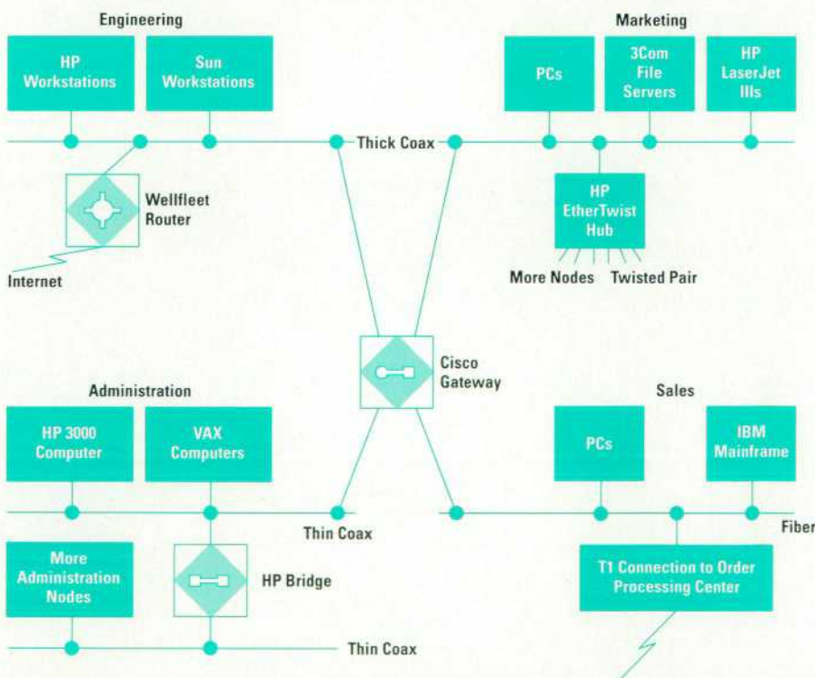
Fig. 1. Acme, Inc.'s hypothetical network.
