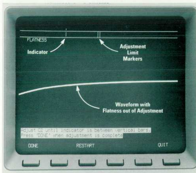
Fig. 4. Flatness adjustment display.
