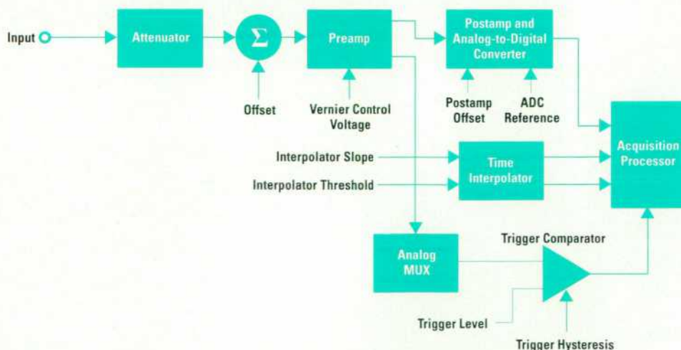
Fig. 1. DAC-generated control voltages in the HP 54601A digitizing oscilloscope.
