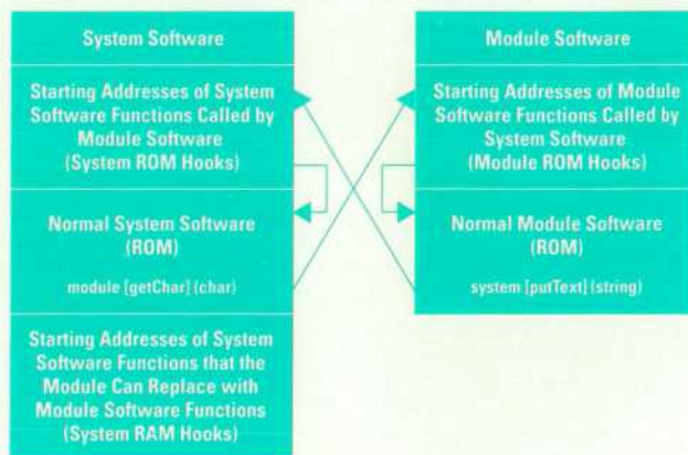
Fig. 3. RAM and ROM look-up tables contain "hooks" that are used for communication between the module software and the software of the system under test.
