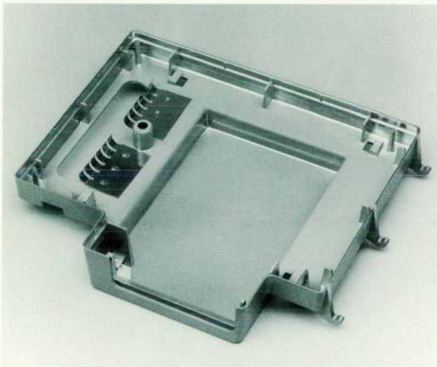
Fig. 4. A finger stock strip is used to reduce the radiated emissions from the option module. The fingers contact the module connector ground shell.
