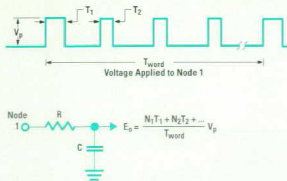
Fig. 2. Filter section input waveform and output voltage.
