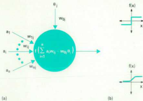
Fig. 2. (a) The structure of a typical neural net node. Inputs are provided by a_1 \dots a_n . Each input has a corresponding weight w_{ij} . The threshold is \theta_j . (b) Two typical output functions f .
