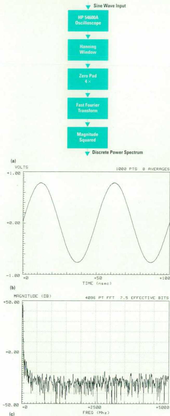
Fig. 6. Discrete power spectrum estimation algorithm. (a) Flow diagram. (b) 20-MHz, 1000-point sine wave from an HP 54600A. (c) Estimated power spectrum using a Hanning window.
