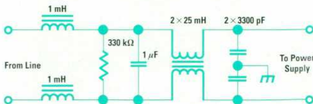
Fig. 7. This is the final circuit used for the switching power supply filter. It will allow the HP 54600 Oscilloscope to meet both FTZ 1046 and MIL-STD-461 conducted emission limits.
