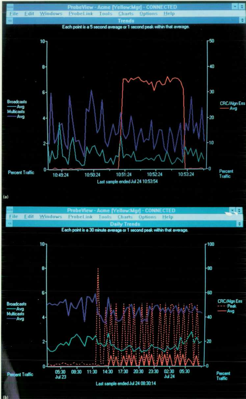
Fig. 3. (a) The trends window shows network activity over the past few minutes. Here the error rate has already dropped back to normal. (b) The daily trends window in this case shows that the error rate has been jumping sharply at even intervals.
