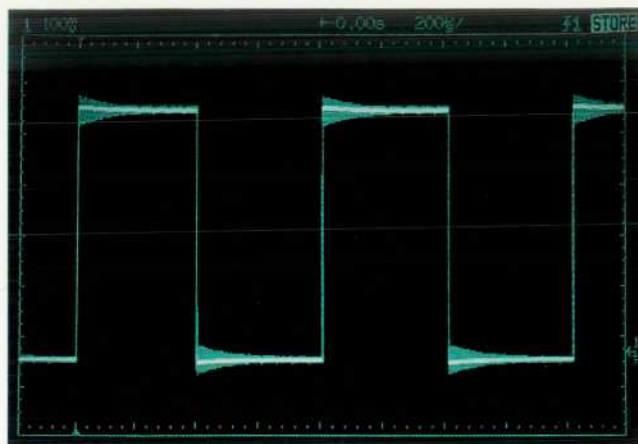
Fig. 2. Minimizing overshoot by adjusting a circuit so that the current live trace at full intensity is always within the autostored historical traces at half intensity.
