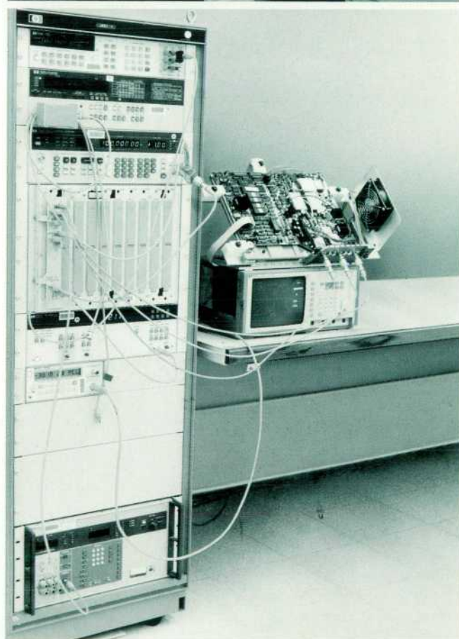
Fig. 9. HP 54600 production test system (top) compared with the test system for an earlier oscilloscope family (bottom).
