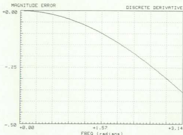
Fig. 2. Frequency response error resulting from the discrete derivative.
