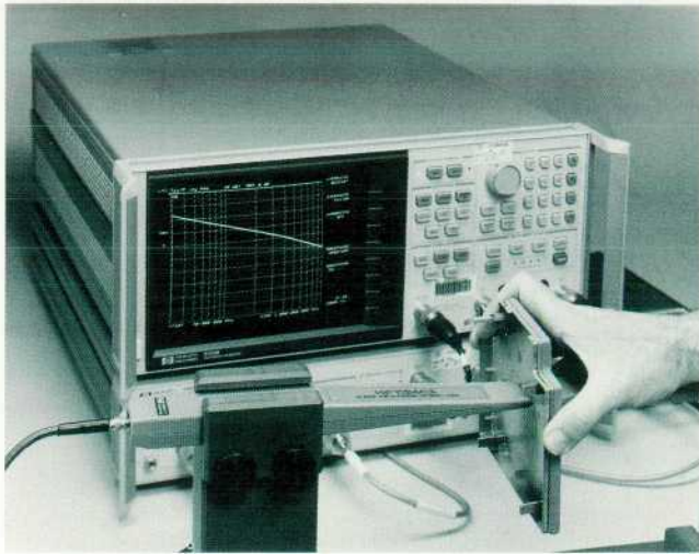
Fig. 2. This photo shows an option module cover being measured using the shielding effectiveness fixture and a network analyzer. This yields a continuous plot of shielding effectiveness versus frequency for thin shielding materials. The technique allows a comparison of different shielding techniques.
