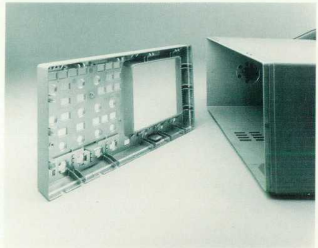
Fig. 1. The main seam that joins the front panel to the cabinet is formed by a knife-edge on the cabinet that fits between a series of raised bumps and stiffening ribs on the front panel. Also see Fig. 7 on page 40.
