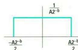
Fig. 1. Probability density function assumed for quantization noise of an ADC with b bits and a range of A .
