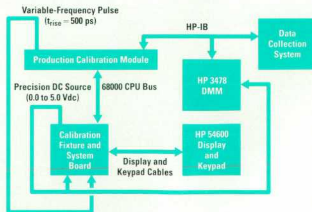
Fig. 1. HP 54600 Series oscilloscope production test system, showing the production calibration module.
