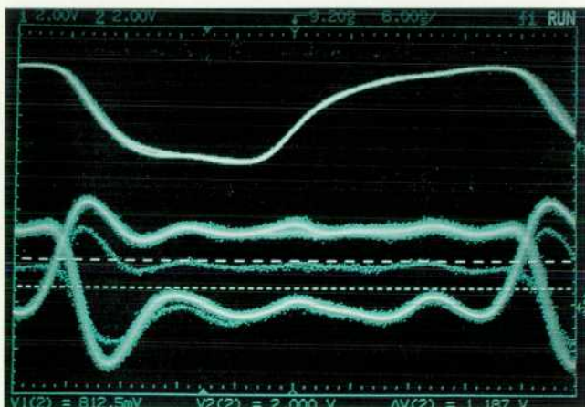
Fig. 5. The upper trace is the read enable signal in a CPU system and the lower traces represent data on the data bus. One of the read cycles resulted in an invalid level on the data bus.
