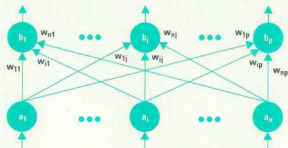
Fig. 3. A two-layer neural net. Input is provided from outside the net to a_1 \dots a_n . Output from the net is provided by b_1 \dots b_p . The weight on the connection between a_i and b_j is w_{ij} .
