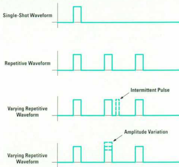
Fig. 2. Waveform types.
