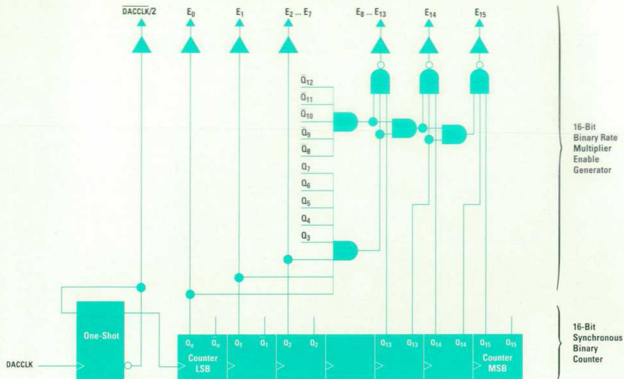
Fig. 6. 16-bit synchronous binary counter and binary rate multiplier enable generator.
