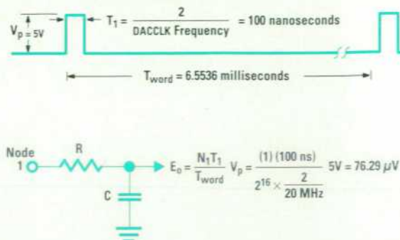
Fig. 3. Filter section input waveform and output voltage for data bit D0 only high, 16-bit data, and a DACCLK frequency of 20 MHz. The input consists of one 5V, 100-ns pulse per T_{word} period.
