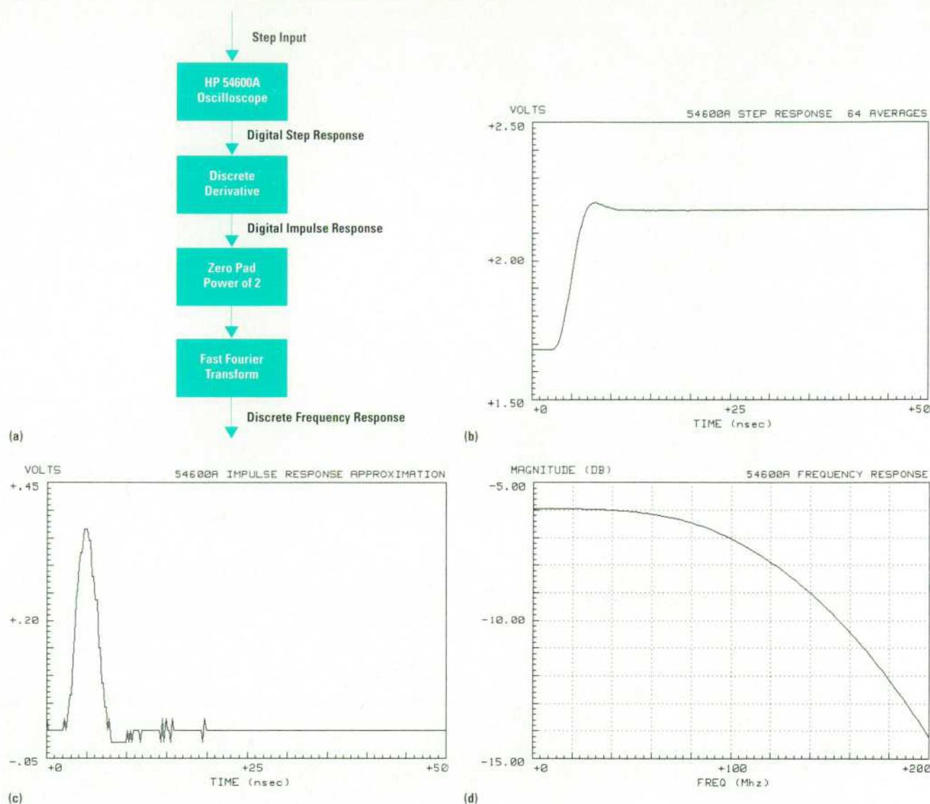
Fig. 1. Discrete frequency response estimation algorithm. (a) Flow diagram. (b) Digital step response of an HP 54600A oscilloscope, channel 1, 100 mV/div. (c) Approximate impulse response using the discrete derivative. (d) Estimated frequency response using a 1000-point step response and 2-GHz sample frequency.
