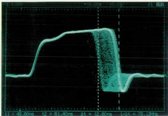
Fig. 4. A jittery signal is shown with the range of jitter at half intensity and the most recent signal at full intensity.
