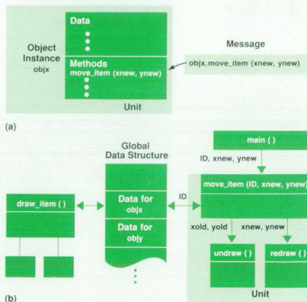
Fig. 1. (a) Object instance objx being sent the message move_item(xnew,ynew) to invoke the method to move a graphical item from one location to another. (b) The same operation being processed in a procedural language environment.
