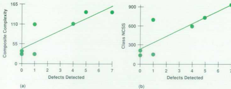
Fig. 8. Defects detected in the classes tested after developers had completed black box testing. (a) Composite complexity versus defects for generic classes tested. (b) NCSS versus defects for the same classes.
