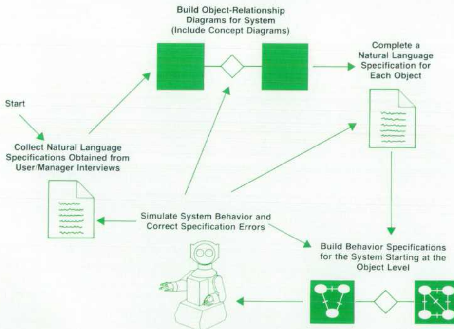
Fig. 11. Process flow for the OSA methodology and the interactions between the object and methodology steps.
