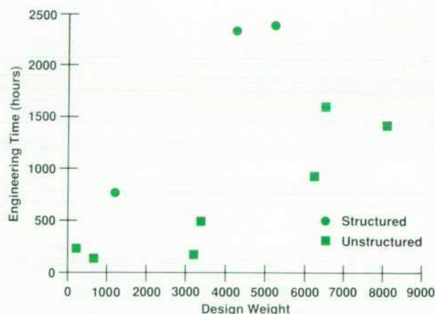
Fig. 2. Engineering hours versus design weight. Design weight is a measure of the effort of coding and testing. It is calculated by an internal tool.
