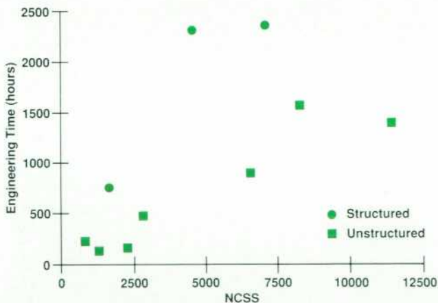
Fig. 3. Engineering hours versus NCSS (noncomment source statements).
