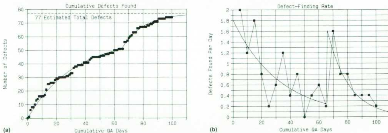
Fig. 2. Project D results. (a) Piecewise curve fit for cumulative defects found m(t) . (b) Piecewise curve fit for defect-finding rate l(t) .
