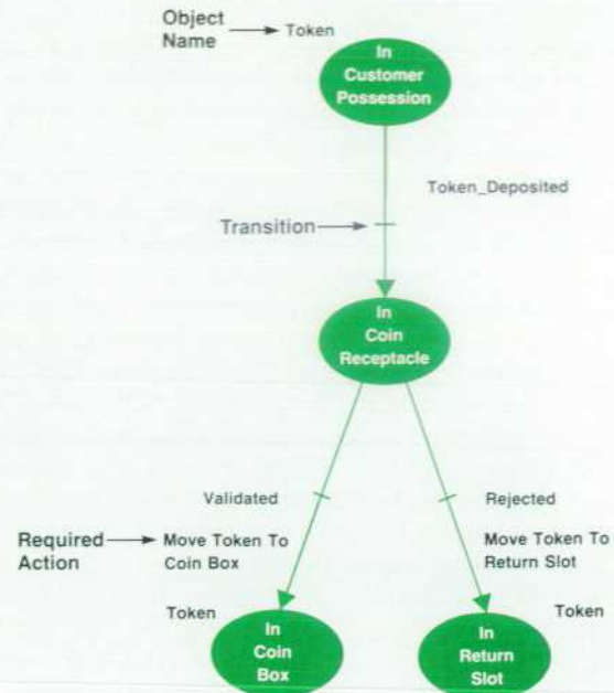
Fig. 10. State net showing the behavior of a token object. When a token is deposited, it transfers from the customer's possession to the coin receptacle. If the token is a valid coin, it is transferred to the coin box as a coin. Otherwise, a rejected token is returned to the return slot as a slug.
