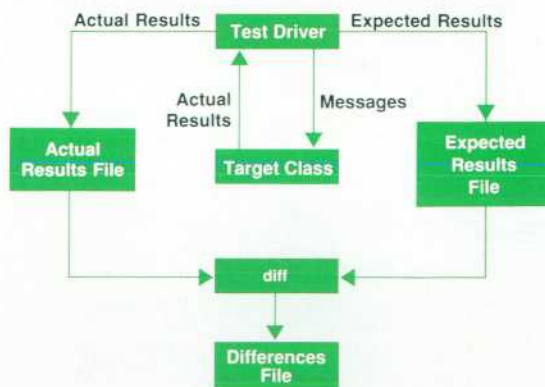
Fig. 6. Data flow diagram for creating verification files and performing the result comparisons.
