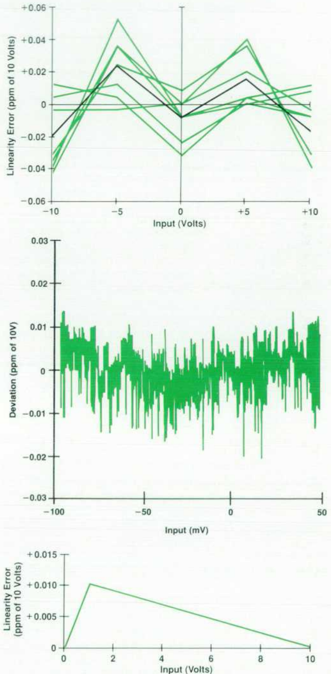
Fig. 4. Results of HP 3458A linearity tests using a Josephson junction array. (a) Seven passes and the average result for linearity error characterization. (b) Differential linearity characteristic. (c) Linearity error for an internal 10:1 ratio transfer.
