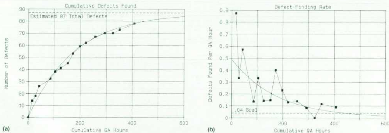
Fig. 1. Project C results. (a) Cumulative defects found m(t) . (b) Defect-finding rate l(t) .
