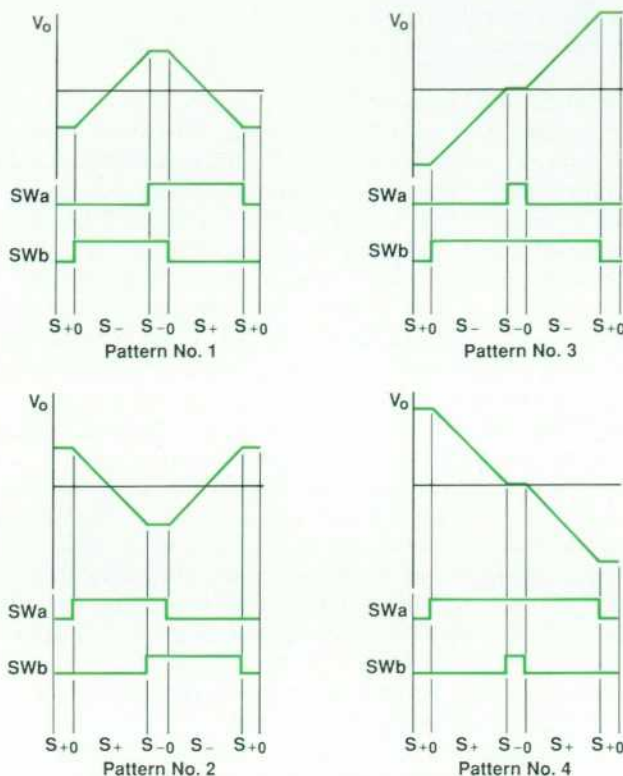
Fig. 7. Multislope rundown patterns for an algorithm that keeps the number of switch transitions constant.
