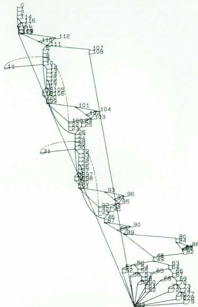
Fig. 5. The program flow graph for a module with a cyclomatic complexity of 36. The high complexity value and the visual presentation indicates that this module is error-prone and very likely hard to maintain.
