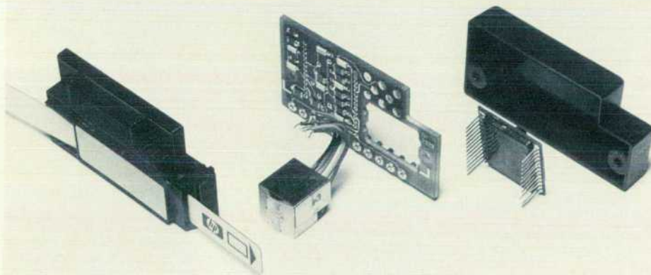
Fig. 3. Exploded view of the optional 82400A Card Reader Module for the HP-71B.
