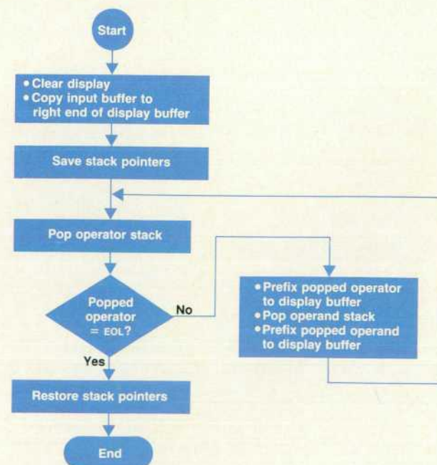
Fig. 2. Decompiler flowchart.
