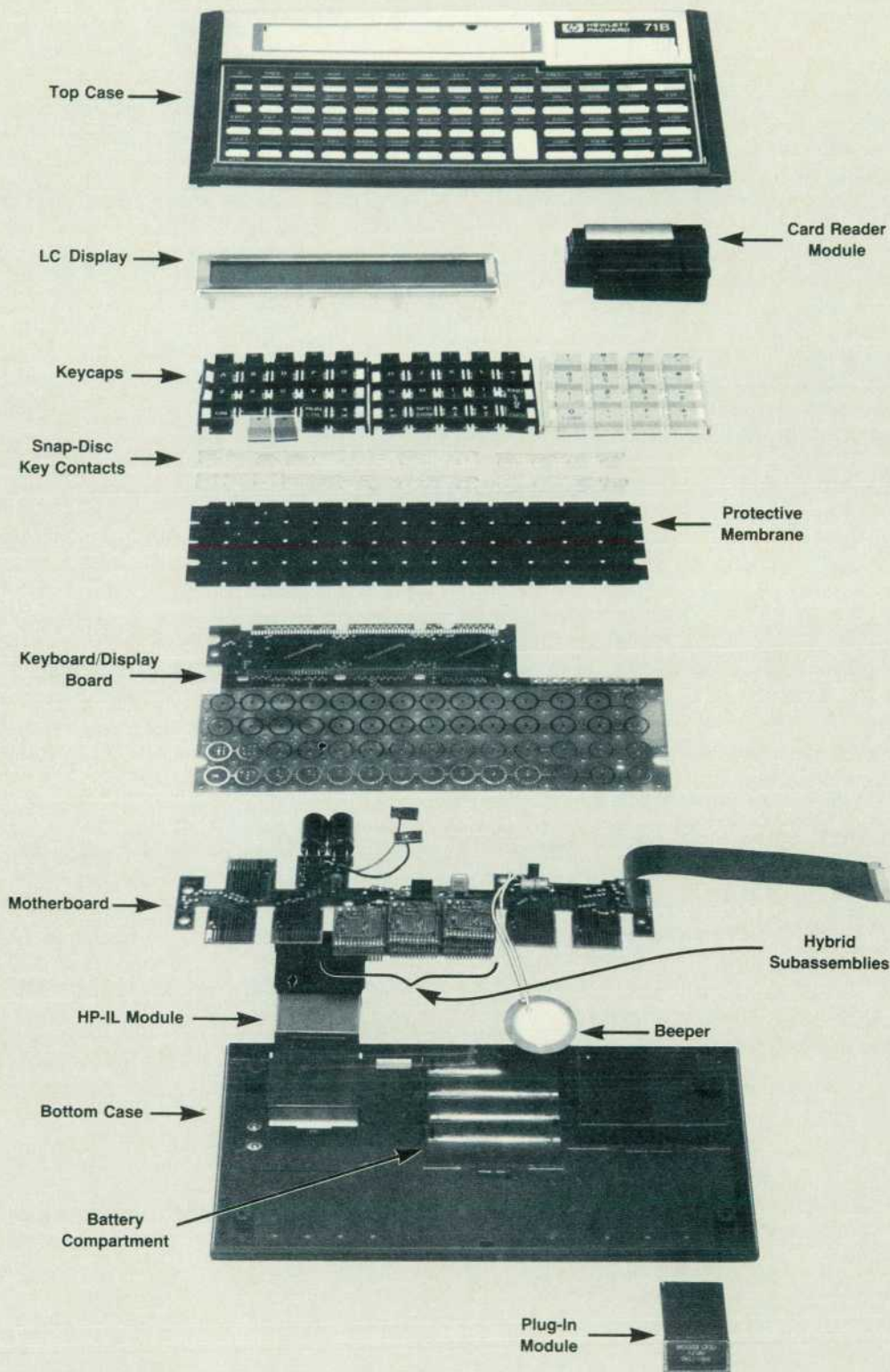
Fig. 1. Exploded view of the HP-71B Computer showing the various packaging features. The mainframe is composed of two subassemblies: the top case assembly and the bottom case assembly. The top case assembly contains the keyboard, display, and CPU and display driver circuitry. The bottom case assembly contains the built-in memory, power circuits, and piezoelectric beeper, and accommodates the optional card reader/recorder and other plug-in modules.
