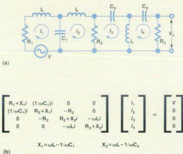
Fig. 2. Example of the ease of use of complex arrays in HP-71B Math Pac matrix operations. To solve for the complex currents in the circuit shown in (a), the complex matrices describing the circuit (b) are entered into the HP-71B and solved using the simple BASIC program listed in the text.
