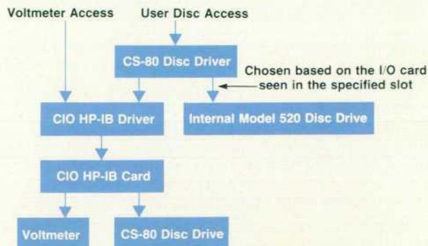
Fig. 2. Driver structure for HP 9000 Model 520 Computer.
