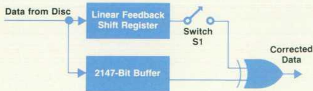
Fig. 1. Circuit for error correction using a Fire code.
