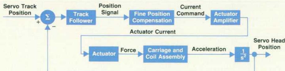
Fig. 1. 7933/35 Disc Drive position control loop block diagram.
