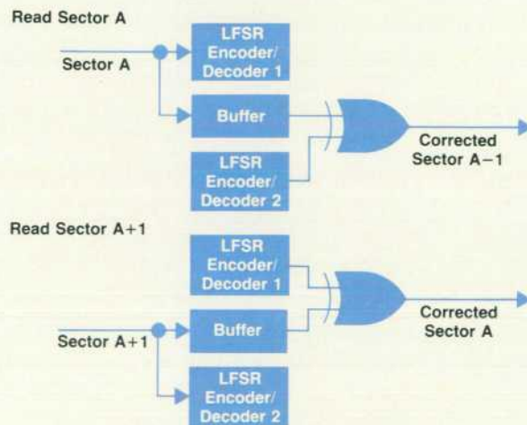
Fig. 2. In the 7933/35 Disc Drives, two linear feedback shift registers are used so that the syndrome for one sector can be generated while the preceding sector is being corrected.
