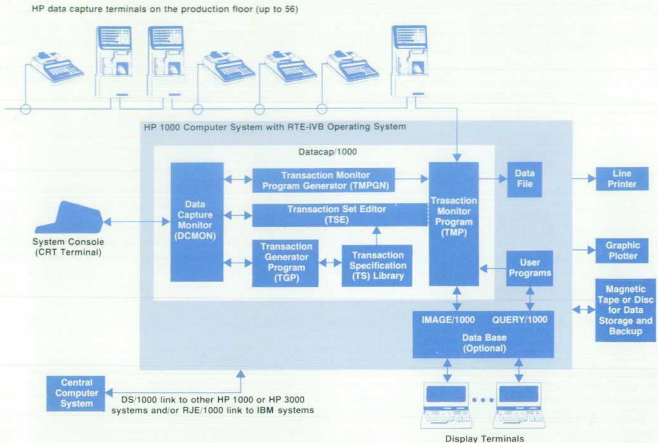
Fig. 3. Major components of DATACAP/1000. The transaction generator program (TGP) and transaction monitor program generator (TMPGN) interactively lead the user through the process of building transaction specifications and the transaction monitor program (TMP). The TMP then manages the collection of factory data and creates data files or enters the data into the IMAGE/1000 data base, if present.
