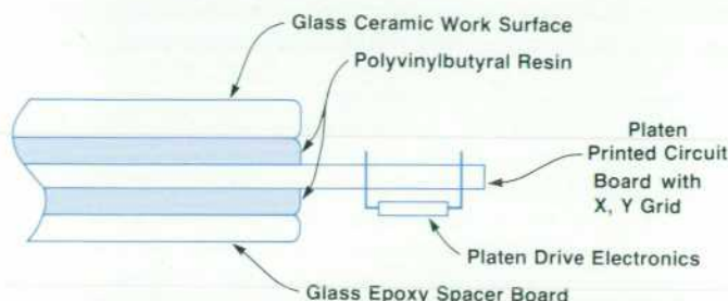
Fig. 5. Cross-section of platen printed circuit board assembly. The ceramic work surface provides a durable layer that resists scratching and is dimensionally stable.
