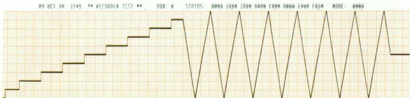
Fig. 2. Stair-step and ramp waveforms are recorded to verify recorder response and linearity. A log of any errors found during extended self-test is also recorded. Errors are indicated by a change in the last three zeros of the status code number(s). An example of a recorder test with no errors is shown above.
