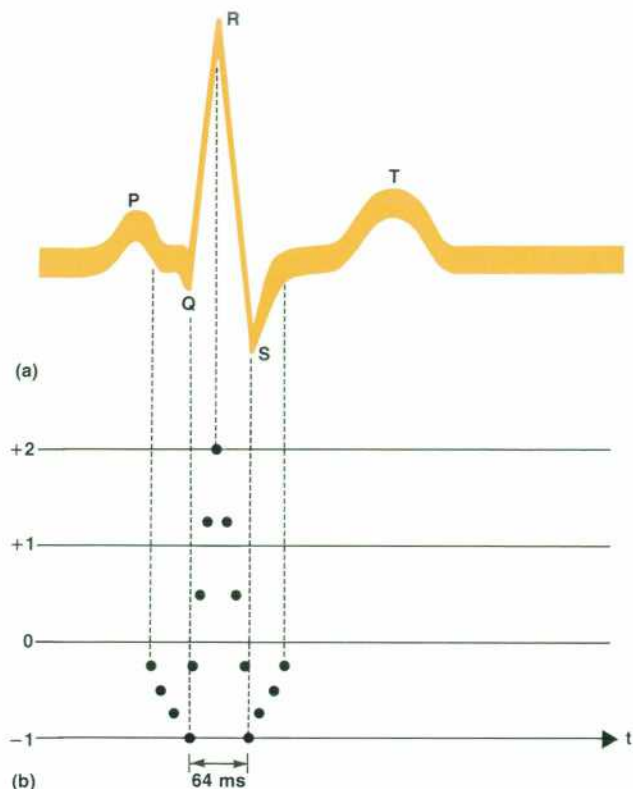
Fig. 1. (a) Typical QRS waveform for one heartbeat. A matched filter processes fifteen 8-ms samples from the ECG waveform. If the samples approximate the values shown in (b) the filter has maximum absolute output.
