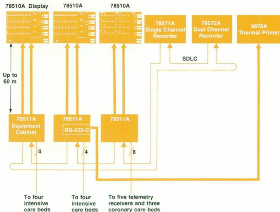
Fig. 7. A typical system application for eight intensive-care patients and eight progressive-care patients sharing one central station location. Two 78502A systems and a 78501A system share two recorders and a hard-copy device. The two-channel recorder is used to record ECG and blood pressure data simultaneously.
