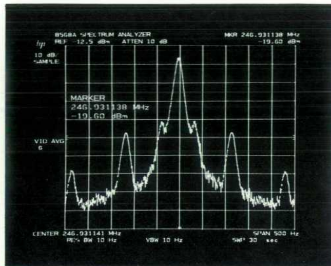
Fig. 5. The trace is sharp everywhere on the CRT. (This is a VHF oscillator test showing 30-, 60-, and 120-Hz sidebands.)
