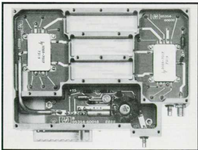
Fig. 3. Switching filter assembly permits rapid acquisition of input signals. 160 \mu s is worst case in automatic mode.
