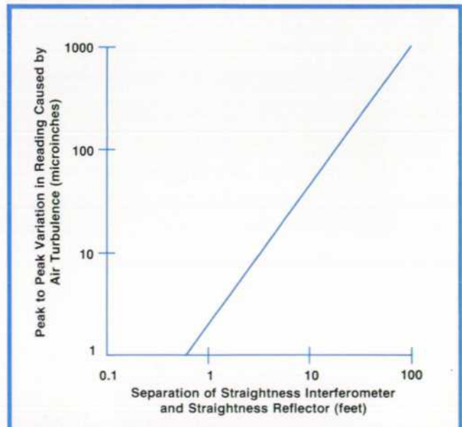
Fig. 5. Air turbulence limits straightness interferometer accuracy by causing random fluctuations in the display. These can be reduced by placing the reflector closer to the interferometer.
