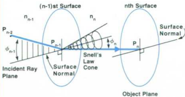
Fig. A. The ray-trace algorithm follows Snell's Law: If n_{n-1} , \phi_{n-1} and n_n , \phi_n are the index of refraction and the angle for the incident and refracted ray, respectively, then n_{n-1} \sin \phi_{n-1} = n_n \sin \phi_n .
