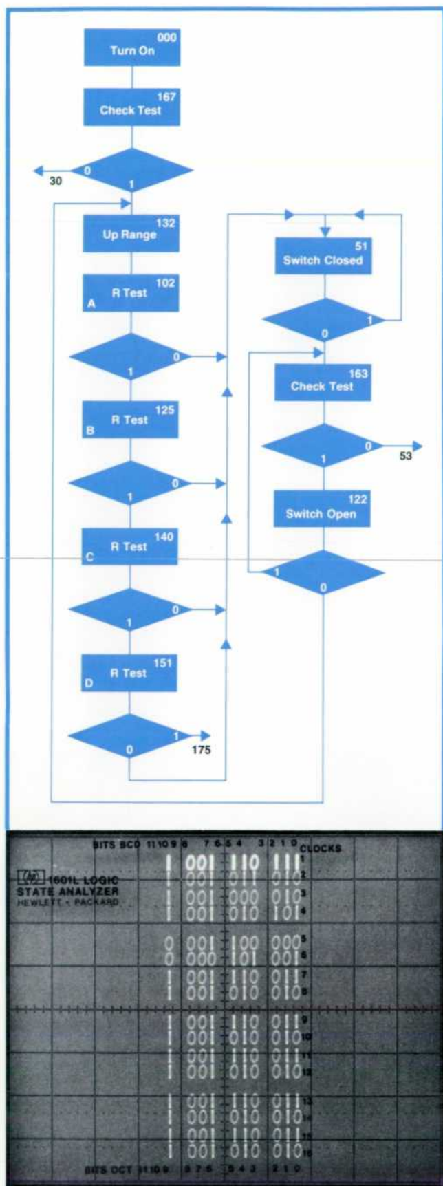
Fig. 4. Program flow in the turn-on sequence of a multimeter is shown by the diagram and the Logic State Analyzer display.
