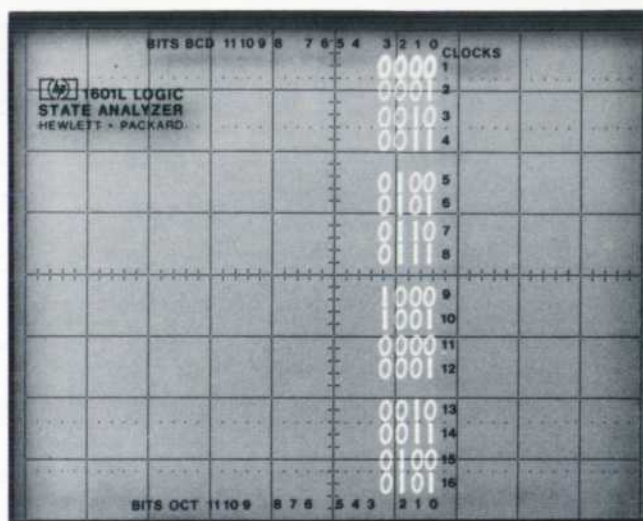
Fig. 3. State flow in a BCD counter. The trigger word at the top is brightened indicating here that the CRT displays the trigger and the 15 states that follow the trigger. The numerical scales, silk-screened on the back side of the contrast filter, assist in identifying states.
