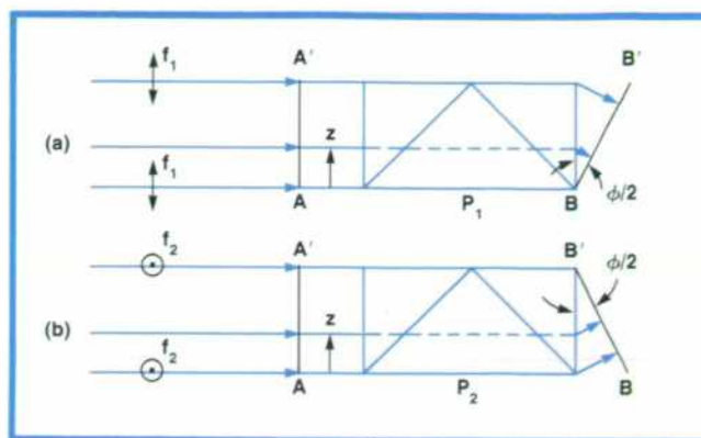
Fig. 3. Optical path difference in the Wollaston prism for f_1 and f_2 is P_2 - P_1 + 2z \sin \phi/2 , where z is the distance from the bottom of the prism and P_2 and P_1 are optical path lengths for z = 0 . A displacement E of the prism in the z direction causes the path difference to change by 2E \sin \phi/2 . This change is measured by the interferometer.
