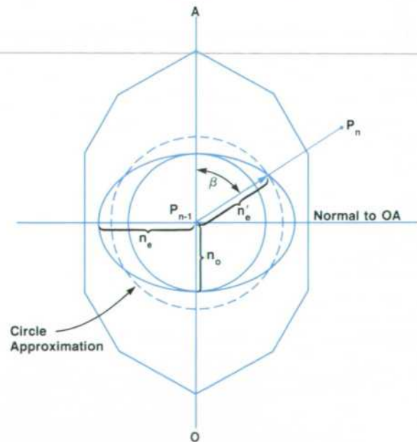
Fig. B. The extraordinary index in a uniaxial material, such as quartz, is a function of the angle between \vec{P}_{n-1} \vec{P}_n and the optic axis and can be approximated using a circle method. The ellipse has rotational symmetry about the optic axis OA.
