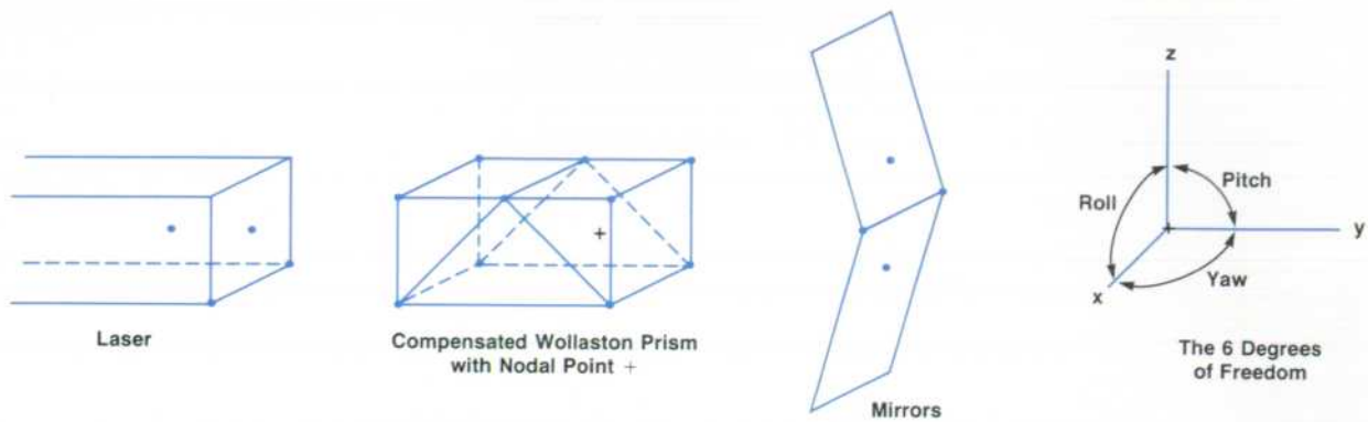
Fig. C. The short-range straightness interferometer program creates a three-dimensional model of the system, using points in space. All movement will occur about a user-defined point.
