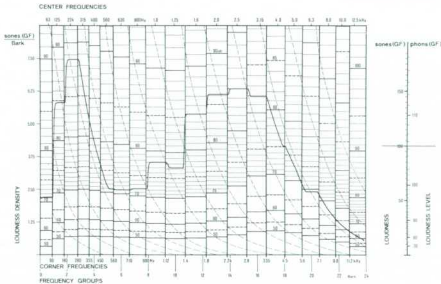
Fig. 2. Typical analysis of the loudness of a single typewriter stroke. (a) Sound pressure waveform has low-frequency components produced by carriage, and large, high-frequency, two-millisecond transient produced by key hitting paper. (b) Loudness analyzer display for typewriter stroke. Total loudness was 100 sones G . (c) Zwicker diagram for typewriter stroke, produced by loudness analyzer while CRT display (b) was being photographed.
