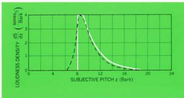
Fig. 5. Loudness density is a quantity which, when integrated over subjective pitch, gives total loudness in sones. (The subscript G indicates a value calculated from a critical-band analysis, as opposed to a subjectively measured value.) This diagram shows a masking curve (dashed line) for a pure 1 kHz tone which has a loudness of 13 sones. The 1 kHz tone excites nerves in the ear as shown by the dashed line. The solid curve is an approximation which has been found to give good results in loudness measurements. The area under each curve is 13 sones.
