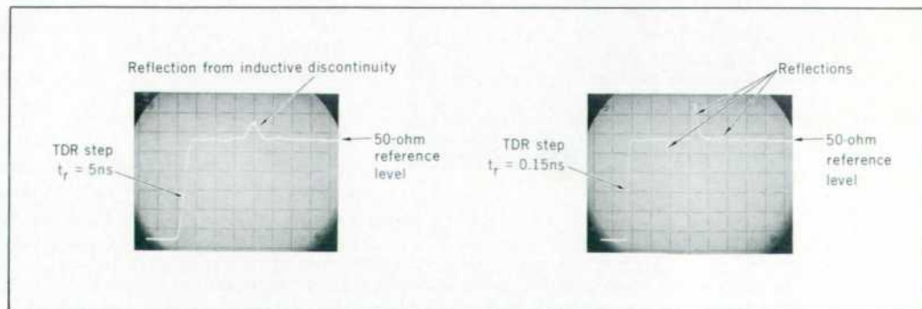
Fig. 3. Oscilloscope displays of TDR displays for typical cable. (a) Since cable will never be used for transmitting pulses with rise times faster than 5 ns, cable is tested with 5-ns rise time converter so that only potentially troublesome reflections appear. (b) Cable response with normal TDR step ( t_r = 0.15 ns). Note additional reflections due to faster rise time.
