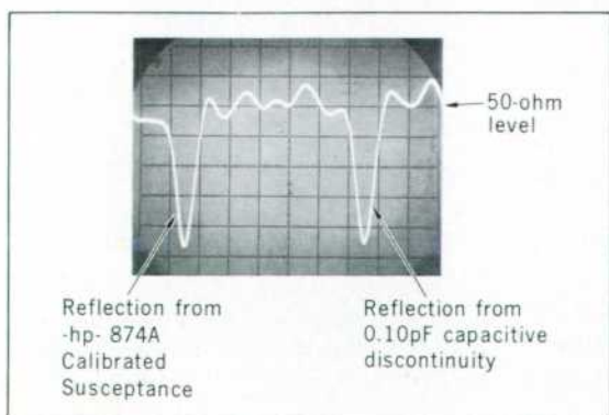
Fig. 4. Oscillogram of portion of TDR display (step not shown) with expanded horizontal and vertical scales, showing reflection from Calibrated Susceptance (l) and reflection from capacitive discontinuity of 0.10 pF (r). Discontinuity was diode across coaxial line. Setup was as in Fig. 3.
