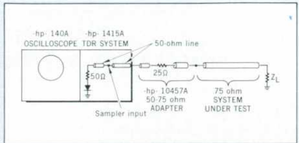
Fig. 2. Block diagram of setup for TDR testing of 75-ohm system using new 50-to-75-ohm adapter. Energy reflected from 75-ohm system is properly terminated by series combination of 25-ohm resistor (adapter) and 50-ohm TDR system, thereby eliminating source re-reflections.
