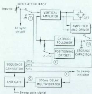
Fig. 1. Simplified block diagram of dc stabilization circuit. During sampling interval, drift sensed at CRT deflection plates, while amplifier input is grounded, charges storage capacitor. Between sampling intervals, stored capacitor voltage is applied to amplifier input to provide offset that cancels drift-induced changes in dc level.
