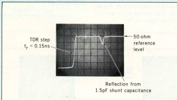
Fig. 1. Oscilloscope display of typical TDR display showing test step ( t_r = 0.15 ns) and reflection from capacitive discontinuity of about 1.5 pF.
