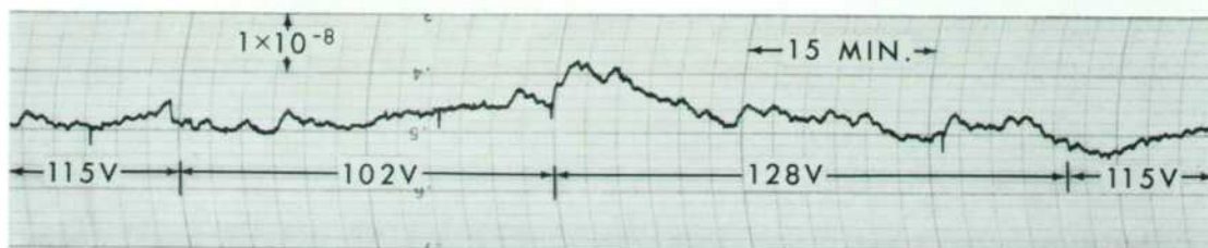
Fig. 6. Typical effect of large line-voltage variations on time-base oscillator stability.
