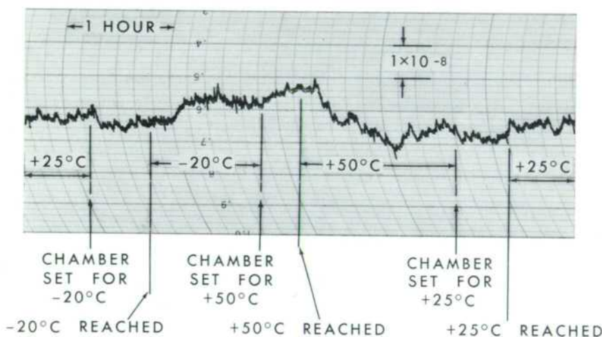
Fig. 10. Record of time-base oscillator stability as complete frequency counter was temperature-cycled in chamber which reached -20^{\circ}\text{C} and +50^{\circ}\text{C} .
