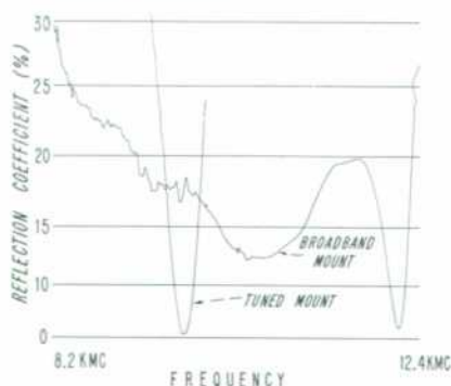
Fig. 2. Record of reflection coefficient magnitude of broadband and tuned bolometer mount. Such permanent records can be made in a minute or two using new sweep oscillator with system described in text.
