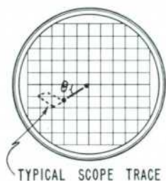
Fig. 7. Representation of typical trace obtained when measuring reflection coefficient magnitude with the setup of Fig. 4. Angle formed with the horizontal by projection of left point of trace thru origin is proportional to reflection coefficient. Position of left point typically varies with frequency because \rho varies. Mask or line drawn on tube face with grease pencil can be used to mark a limit for production acceptance tests.
