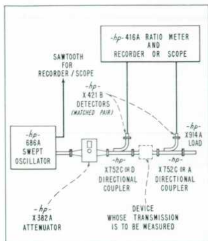
Fig. 5. Equipment arrangement for measuring attenuation, gain, isolation or other transfer characteristics.
