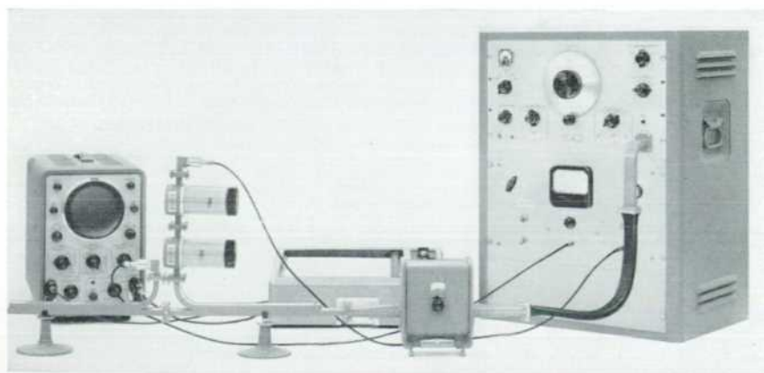
Fig. 3. Complete setup for measuring magnitudes of reflection coefficient and transfer characteristics either in permanent record form or as viewed on scope.
