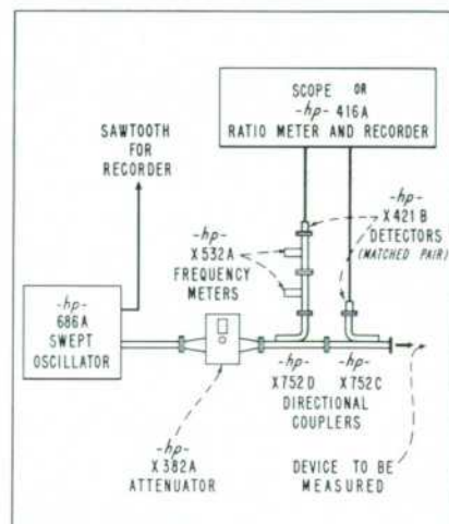
Fig. 4. Equipment arrangement for measuring reflection coefficient magnitude in either permanent form or as viewed on meter or oscilloscope trace. Wavemeters in incident arms are used to insert marker pips at desired points.
