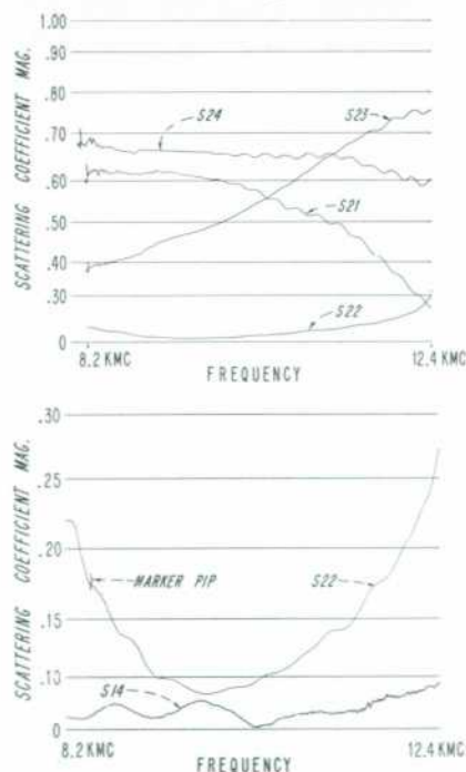
Fig. 6. Records made of magnitude of scattering coefficients of hybrid-tee using arrangements of Figs. 4 and 5. Arms 1 and 4 are H and E arms, respectively, 2 and 3 the side arms. Such records can be made in only a few minutes. Marker pips are from wavemeters and can be used to define frequency ranges of special interest.
