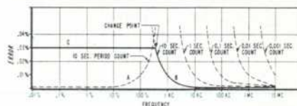
Figure 6. Accuracy curve of Model 524A Frequency Counter for direct frequency and period measurements.
