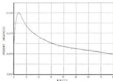
Figure 7. Warm-up stability curve of -hp- Model 608A 10-500 mc signal generator with frequency dial set for 10-megacycle output. Measurements made with -hp- Model 524A at 20-second intervals.
