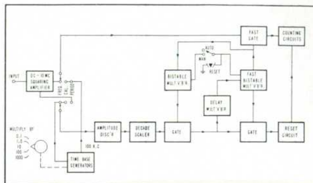
Figure 8. Block diagram of -hp- Model 524A Frequency Counter.
