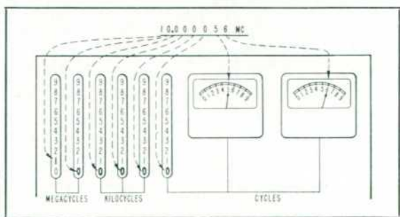
Figure 1. Display arrangement of new -hp- Model 524A Frequency Counter. Columns of neon tubes behind panel slots illuminate the proper numerals which are reverse-printed on transparent plastic. Example shown represents a frequency of 10,000,056 cps counted for period of one second. Maximum rate for instrument is 10 mc; maximum counting period is 10 seconds.
