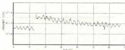
Figure 4. Measured stability curve of 10 mc oscillator turned off for one minute after 13 minutes.
