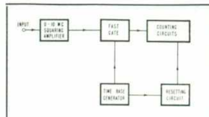
Figure 3. Basic block diagram of -hp- Model 524A Frequency Counter.
