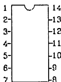
MC1488 MC1489
